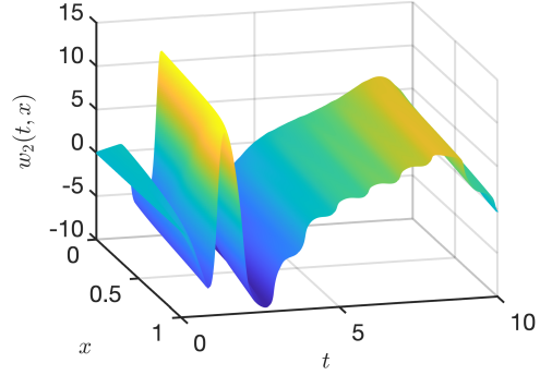
FIG. 6. Solution w_2(t, x) to (6.1) for 0 \leq t \leq 10 and for 0 \leq x \leq 1 .
