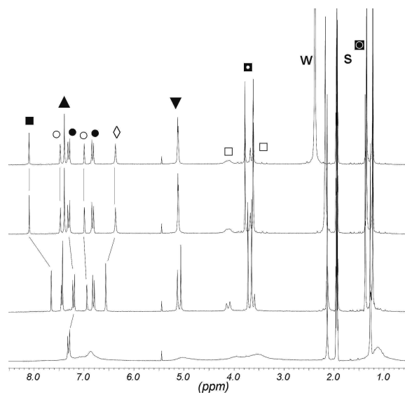
Figure 2. 1 H NMR (CD 3 CN, 300 K) of the titration of calixarene 4 with Zn(OH 2 ) 6 (ClO 4 ) 2 . From bottom to top: before and after addition of 1, 2.25 and 4 equiv of Zn(II). ■ H triazole , ○ H Im , ▲ H ArBu , ● H ph , ◇ H Artria , ▼ OCH 2 and CH 2Im , □ CH 2 Ar, ■ OCH 3 and NCH 3 , ■ t Bu
