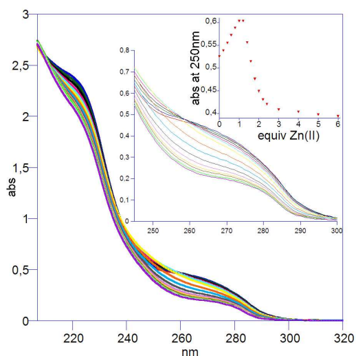
Figure 1. UV-vis titration of calixarene 4 (3.10 -5 M in CH 3 CN containing 10 mM Bu 4 NClO 4 , T = 293 K) with Zn(OH 2 ) 6 (ClO 4 ) 2 .
