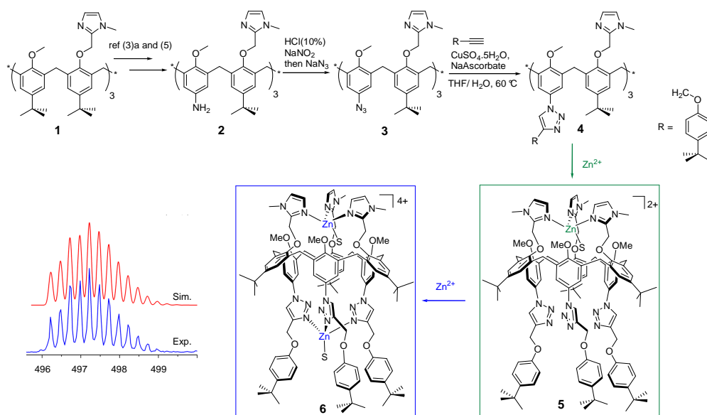
Scheme 1. Synthesis of the triazole calixarene 4 , the monometallic zinc complex 5 and the bimetallic zinc complex 6 .
