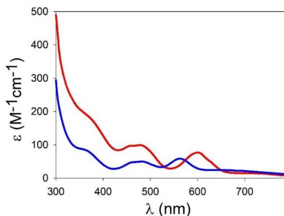
Figure 2. UV-Vis spectra (in CH 3 CN/CH 2 Cl 2 1:1 v/v) of 1 (red) and 2 (blue).
