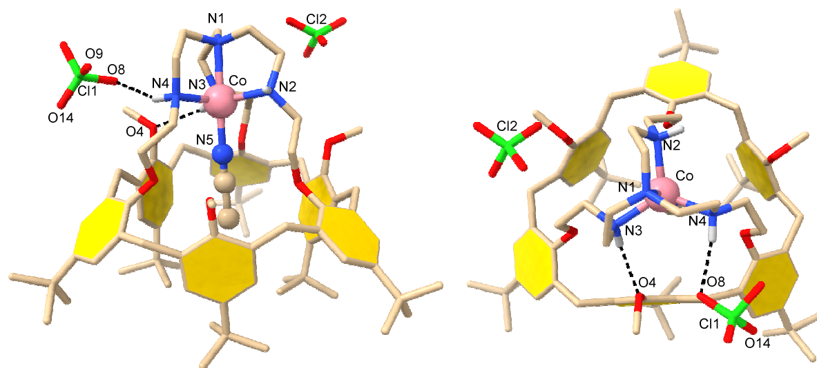
Figure 3. Side and top views of the crystal structure of 1 . Hydrogen bonds are indicated by dashed lines. H-atoms, except polar ones, are omitted for clarity.
