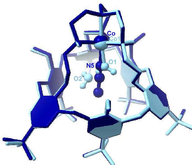
Figure 6. Overlap of the crystal structures of 1 (dark blue) and 1' (pale blue). H atoms, except polar ones, are omitted for clarity. Atoms of the intra-cavity guests are represented in ball-and-stick style.
