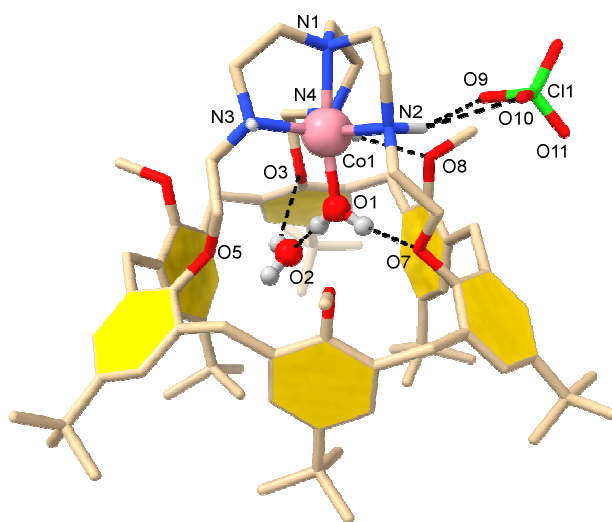
Figure 4. Crystal structure of [\text{Co}^{\text{II}}(\text{OH}_2\cdots\text{OH}_2)\text{Calix-TREN}^{\text{Me}}][\text{ClO}_4]_2 ( 1' ). Hydrogen bonds are indicated by black dashed lines. H-atoms, except polar ones, are omitted for clarity. Only one counterion is represented as the second one is highly disordered.
