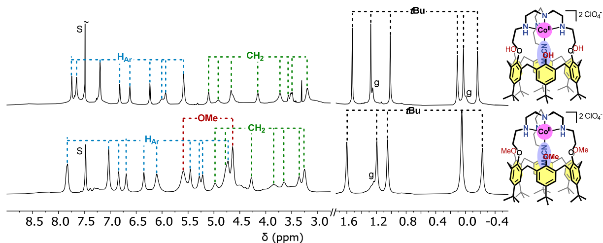
Figure 1. Regions (+2.5 to +9.5 ppm and -0.55 to +1.75 ppm) of the ^1\text{H} NMR spectra of 1 (600 MHz, 298 K) (bottom), and of 2 (500 MHz, 298 K) (top) in \text{CD}_3\text{CN}/\text{CDCl}_3 1:1. The methylene protons detected here are part of the calixarene core, part of the TREN cap. Additional peaks are observable in the low-field region (+300 to +10 ppm) (see the SI), but some protons could not be detected. The t Bu region (-0.55 to 1.75 ppm) is unzoomed 8 times. “S” stands for \text{CHCl}_3 and “g” for grease.
