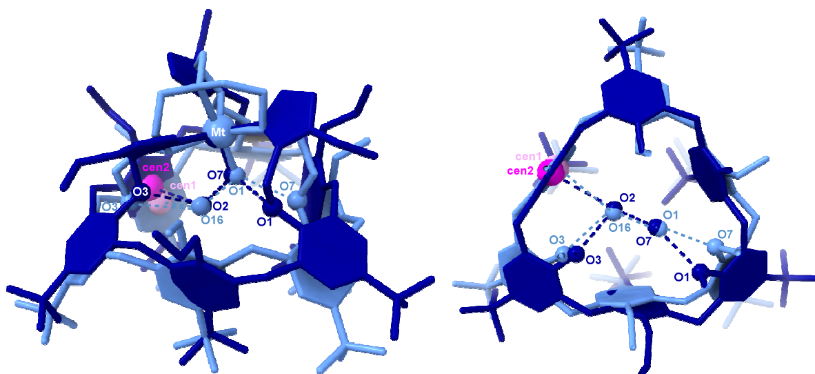
Figure 5. Side and top views of the overlap of the crystal structures of previously reported tris(N-ethylimidazol)calix[6]arene Zn-aqua complex (dark blue) and of 1' (pale blue). In the top view, the small rim substituents have been removed for clarity. Counter anions as well as H-atoms are omitted for clarity. Intracavity water molecules, as well as atoms involved in the non-covalent interactions with them are presented in ball-and-stick style and labelled. The purple spheres represent the centroids (cen1 and cen2) of the aromatic units involved in OH \cdots \pi interactions. Mt = Co ^{2+} or Zn ^{2+} .
