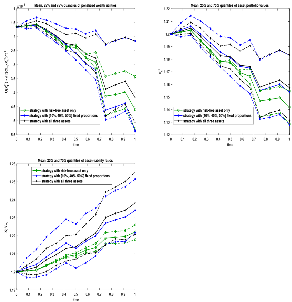
Figure 3. Empirical mean: 25% and 75 % quantiles of the penalized utilities of wealth ( upper left ), asset values ( upper right ), and asset-liability ratios ( bottom ) when using the risk-free asset only, when using fixed proportions invested in the three considered assets (10% in the risk-free asset, 40% in the default-free bond, and 50% in the default-sensitive bond), and when using the optimal proportions in the three assets as solution of (27).
