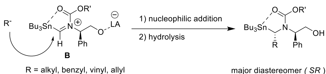
Scheme 4
