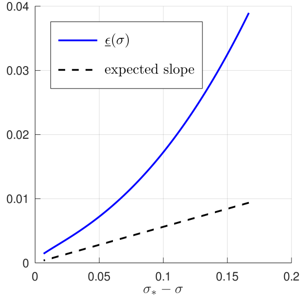
FIGURE 5. Dependence of \underline{\epsilon}(\sigma) (solid curve) and the asymptotic approximation \epsilon_0(\sigma) (dashed line) versus \sigma \in [0.5, 0.66] for d = 5 .
