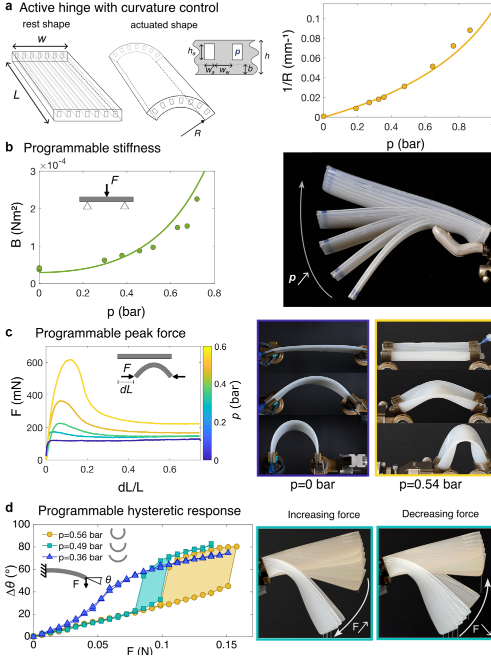
Figure 5. Active hinge inspired by the petiole base. (a) The elastomeric structure contains off-centred airways along its length, that produces unidirectional curvature when pressurised. Curvature as a function of pressure for a structure with L = 100 mm, w = 32 mm, h = 2.7 \pm 0.1 mm, b = 0.55 \pm 0.1 mm, h_a = 1.15 \pm 0.05 mm, w_a = 0.85 \pm 0.05 mm, w_w = 1.15 \pm 0.05 mm, E = 550 \pm 20 kPa and \nu = 0.5 . Circles correspond to experiments and the solid line to the model without any fitting parameter (Eqs. (2) and (3)). (b) Programmable stiffness: when the pressure is increased, the transverse curvature induces a strong bending stiffening, such that the structure may sustain its own weight. Bending modulus, measured with a 3-point bending test, as a function of the inner pressure. Circles correspond to experiments and the solid line to the toy model (Eq. (B.1)), inferring the curvature computed in (a). (c) The nonlinear response may be also programmed. Upon compression, the structure buckles and exhibits a peak force that strongly varies with the transverse curvature and hence the inner pressure. Beyond this point, the force decreases to reach a plateau, that barely varies with the applied pressure. (d) Programmable hysteretic response: cantilever experiment in which the end force is gradually increased and then decreased. As pressure is increased within the structure, it transitions from a smooth to a discontinuous behaviour with two jumps for the final orientation \theta , exhibiting a hysteretic loop that increases in size with the applied pressure. (right) Overlay of pictures with a regularly increasing (resp., decreasing) force, corresponding to the green curve, highlighting the sudden jump in orientation. For (c) and (d), structure with w = 50 mm, h = 2.6 \pm 0.1 mm, b = 0.6 \pm 0.1 mm, h_a = 1 \pm 0.05 mm, w_a = 0.8 \pm 0.05 mm, w_w = 1.2 \pm 0.05 mm, E = 550 \pm 20 kPa and \nu = 0.5 . L = 120 mm for (c); for (d), L = 105 mm (yellow curve); L = 80 mm (green curve); L = 60 mm (blue curve).
