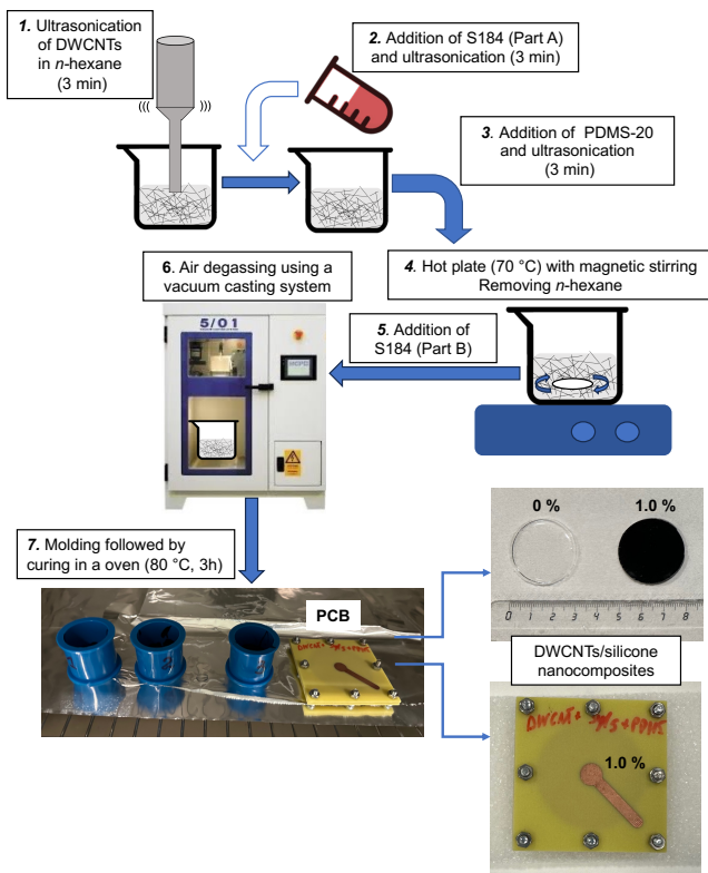
Fig. 1. Schematic diagram of the DWCNTs/silicone nanocomposites preparation steps.
