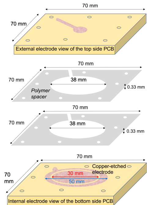
Fig. 2. Schematic representation of a printed circuit board (PCB) sandwich structure.
