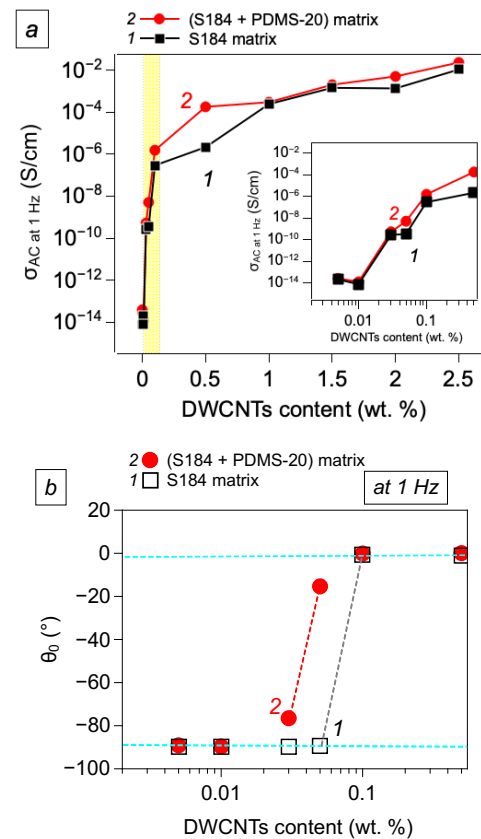
Fig. 4. (a) Electrical conductivity ( \sigma_{AC} ) at 1 Hz vs DWCNTs content for both studied DWCNTs/silicone nanocomposites. The inset shows a log–log plot for the yellow box part, where the percolation threshold occurs; (b) Phase shift ( \theta_0 ) of the impedance response for both silicone-based nanocomposites vs DWCNTs content at 1 Hz.
