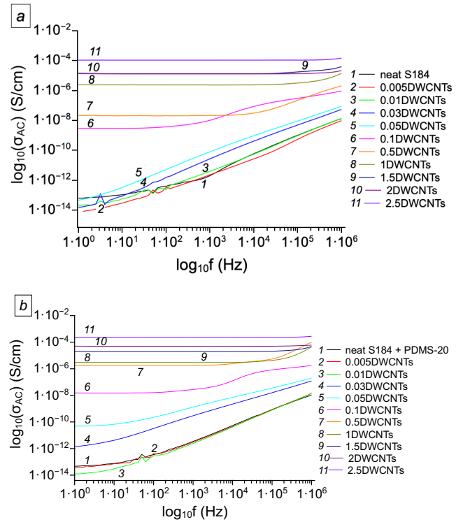
Fig. 3. Variation of AC electrical conductivity with frequency, for the different DWCNTs contents based on (a) S184 and (b) (S184 + PDMS-20) silicone matrices.
