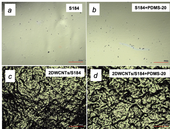
Fig. 6. Optical surface micrographs of neat silicone matrices (a,b) and polymer nanocomposites filled with 2.0 wt.% DWCNTs (c,d) with \times 5 and 500 μm resolution.
