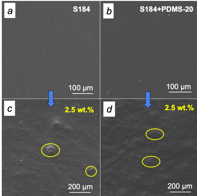
Fig. 5. SEM images of top-view for neat silicone matrices ( \times 500 , a,b) and polymer nanocomposites filled with 2.5 wt.% DWCNTs ( \times 200 , c,d). Yellow circles indicate what we assume to be DWCNTs agglomerations.
