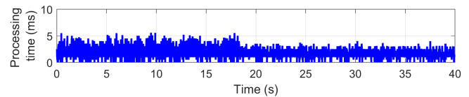
Fig. 7. Processing time of Diff-UIO under Test 3.
