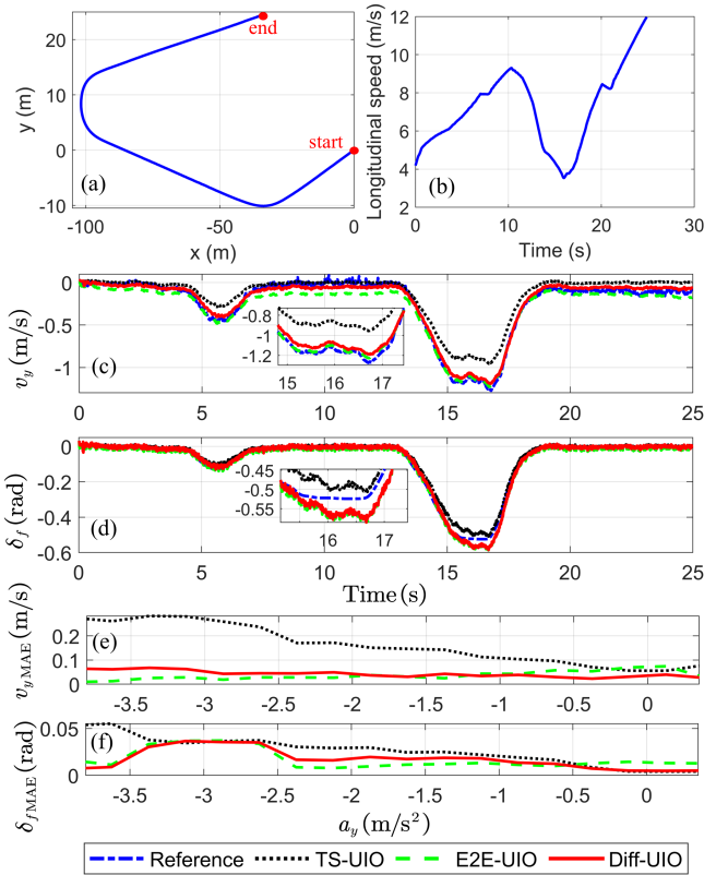
Fig. 9. Estimation results of Test 2: (a) Vehicle path, (b) Longitudinal velocity v_x , (c) Lateral velocity v_y , (d) Steering angle of the front wheel \delta_f , (e) MAE of v_y , (f) MAE of \delta_f . (Binsize=0.25m/s 2 , 130% SSM parameter m, I_z scaling).
