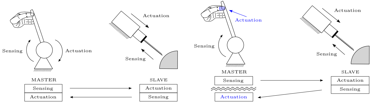
(a) Common approach for teleoperation systems. The force fed back to the user is applied directly on the end-effector of the master device, which is also in charge of steering the slave robot. A control action is needed to avoid instability.
