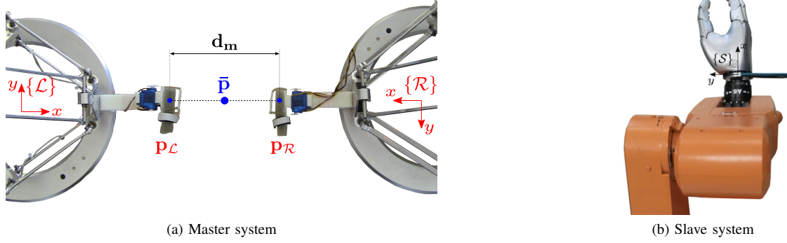
Fig. 8. Peg-in-hole in a real (teleoperated) environment. \{\mathcal{L}\} and \{\mathcal{R}\} are two reference frames on the Omega haptic interfaces and \bar{\mathbf{p}} is the point located between the two end effectors. Figure (b) shows the origin of the slave reference frame \{\mathcal{S}\} , that is placed on the robotic hand wrist.
