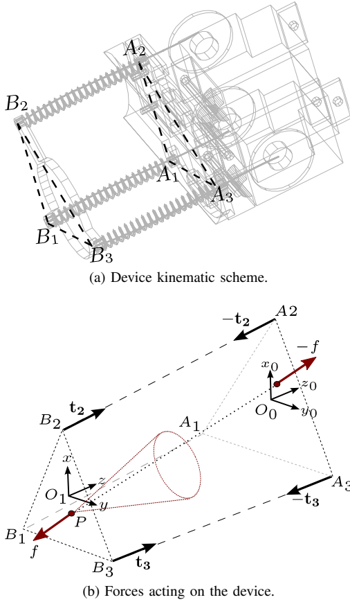
Fig. 3. The 3-DoF cutaneous device model. In (a), A_i and B_i are the points where the cables link the static and mobile parts of the device, respectively. In (b), force \mathbf{f} is applied by the fingertip to the device at point P . Its direction has to be inside the friction cone (in red) in order to fulfil our friction constraint. On the other hand, \mathbf{t}_i represent the forces applied by the actuators to the mobile platform.
