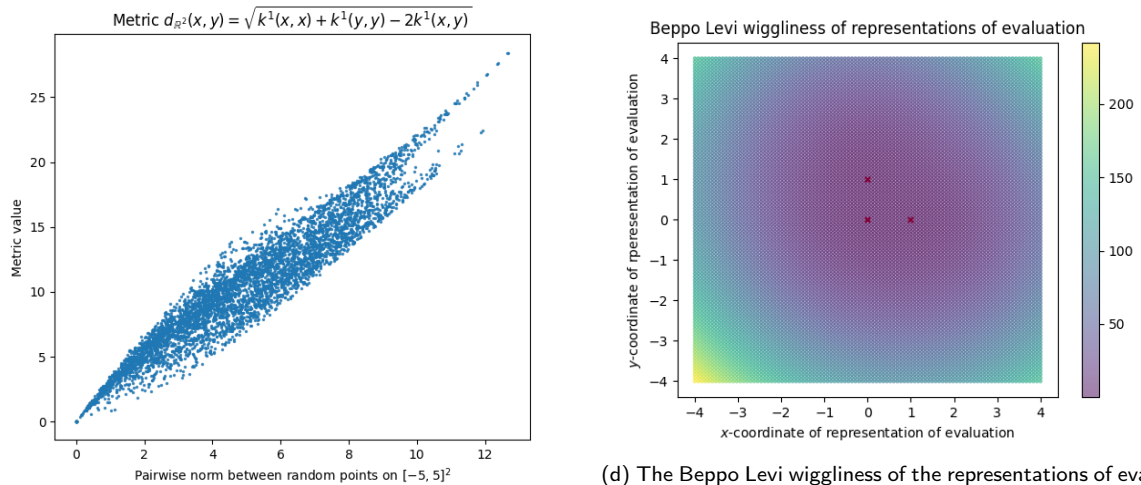
(c) k^1 involves a relatively sensible notion of distance on the index set, though it is influenced by proximity to the unisolvent set. (d) The Beppo Levi wiggleness of the representations of evaluation at a point vary substantially with the distance of the point to the unisolvent set. This is troubling as the unisolvent set is chosen independently of the data we wish to interpolate.
