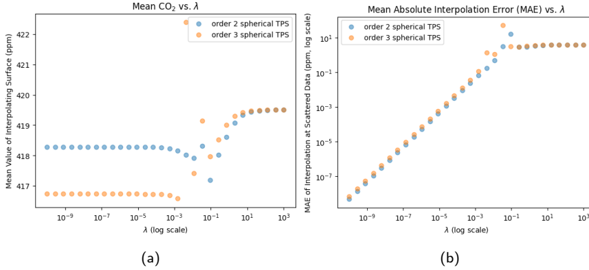
Figure 8: (a) A plot of the global mean CO 2 of the interpolating surface as a function of the regularization parameter \lambda used in constructing it. With low values of \lambda , the order 2 and order 3 spherical splines interpolate the data and, due to their different wiggleness penalties, form different interpolating surfaces with different mean concentrations of CO 2 to do so. With high values of \lambda , the order 2 and order 3 spherical splines agree, as they each yield what is effectively an element of \mathcal{H}_0 = \text{span}\{1\} due to the excessive penalty imposed on wiggleness. With high, but not excessive values \lambda , erroneous averages may be found. (b) The mean absolute error in interpolation at the data points increases with the regularization penalty \lambda , until the interpolation surface is essentially constant.
