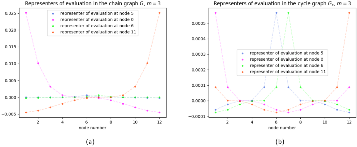
Figure 4: (a) plots the representers of evaluation in \mathcal{H}_1 (with order m = 3 ), i.e. k_t^1 = k^1(\cdot, t) , of the kernel k^1 associated with the chain graph G (shown in Figure 2) on \mathcal{X} = \{1, \dots, 12\} at t = 1, 6, 7 , and 12. (b) gives the same, but for the kernel associated with the cycle graph G_c (shown in Figure 3). In both cases, all edges assume the same weight (12). Dashed lines interpolating between the nodes are included as a visual aid but carry no meaning.
