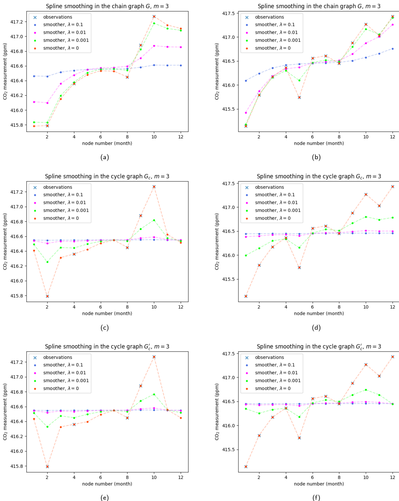
Figure 5: For four distinct choices of wiggleness penalty parameter \lambda , (a), (c), and (e) give the smoothing splines after observing nodes \{2, 4, 8, 9, 10\} ; (b), (d), and (f), after observing all nodes 1-12. The top row corresponds to the chain graph G (Figure 2, all edge weights 12); the middle, G_c (Figure 3, edge weights 12); and the bottom, G'_c , which is G_c but with w(t_1, t_{12}) set to 144 to further penalize the non-periodicity of the smoothing splines (though a constrained optimization or smooth-periodic decomposition can be applied).
