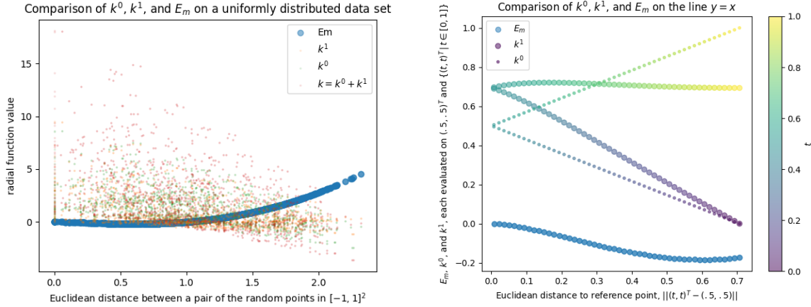
(a) E_m , k^0 , and k^1 evaluated pairwise on points placed uniformly in [-1, 1]^2 , using the unisolvent set of Example 2.69. (b) E_m and k^1 evaluated on y = x , compared to a fixed reference (0.5, 0.5)^T . Clearly k^0 and k^1 are not radial.
