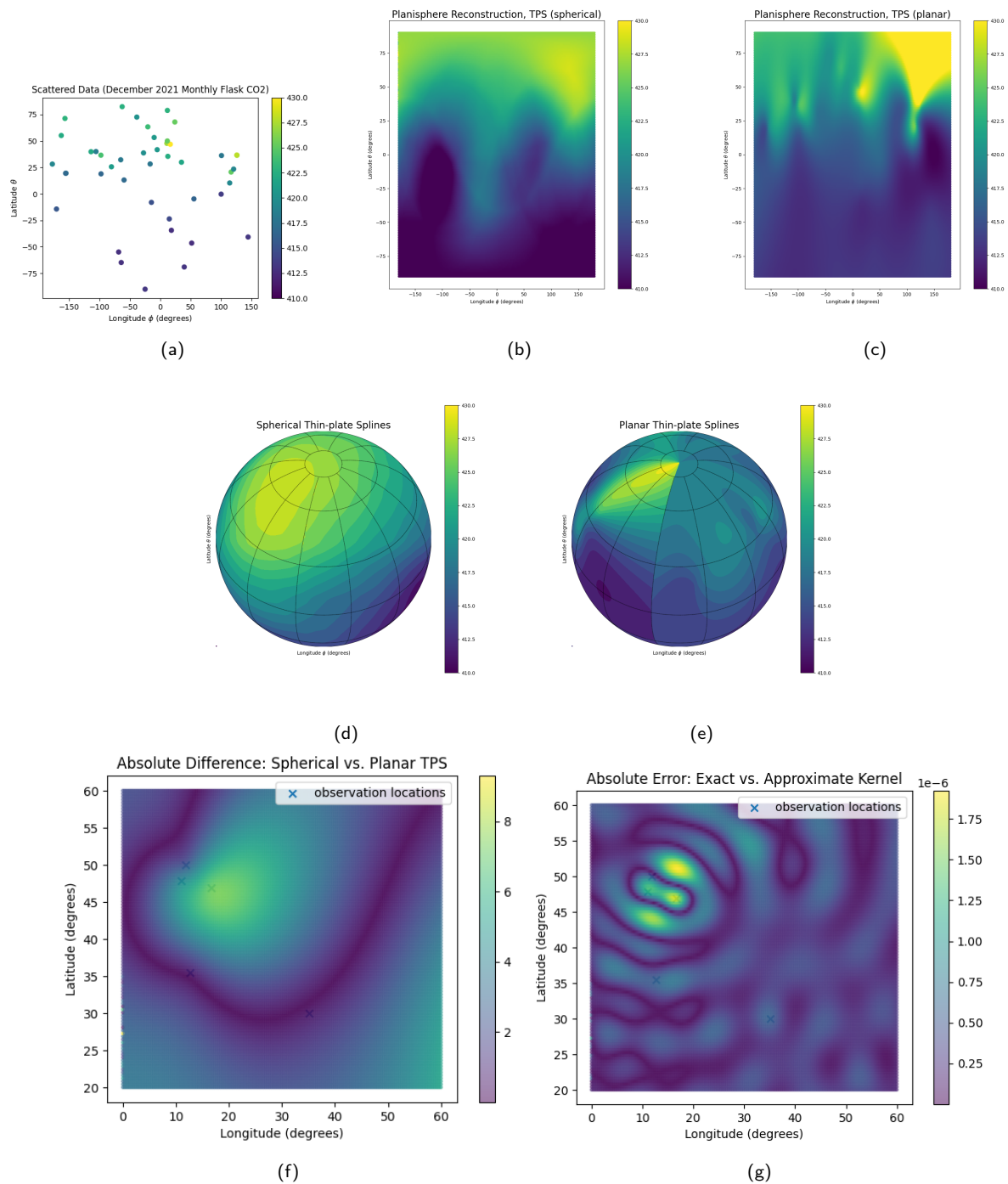
Figure 7: (a) Scattered data of December 2021 monthly averages of flask-air CO 2 readings at 44 sites in the Global Monitoring Laboratory network 57 . (b)-(c) Spherical and planar thin-plate spline fits of these data, respectively, both of order 2. The spherical thin-plate spline interpolant is more coherent with the geometry of the sphere. The planar interpolation surface lacks longitudinal periodicity and embarks on a mean-altering but wiggleness-minimizing excursion beyond the sample points in the top-right corner of (c) . (d)-(e) display samples of the same surfaces as in (b)-(c) , respectively, but these sample points, uniformly spaced in the plane under an equirectangular projection, are mapped back onto a sphere, which throws into relief the meridional discontinuity of planar thin-plate interpolating surface. In the top-right corner of (c) , the interpolating surface, outside the convex hull of the planar control points, loses its curvature. (f)-(g) show the differences between the spherical and planar thin-plate splines, trained on all 44 points, in their reconstruction of a mesh of points between 0° E and 60° E longitude, and 20° N and 60° N longitude.
