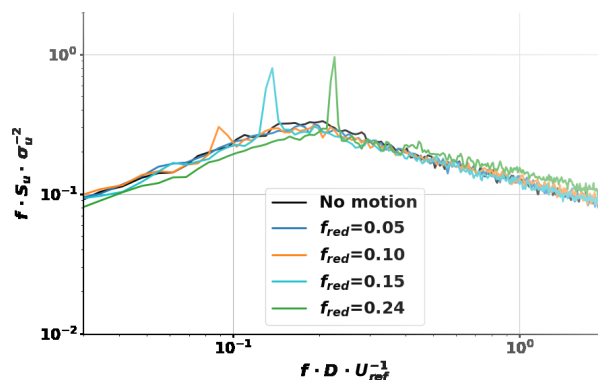
Figure 7: Spectra of the longitudinal velocity component at hub height. Constant amplitude, varying f_{red} . Measured 4.6 D downstream of the actuator disc.
