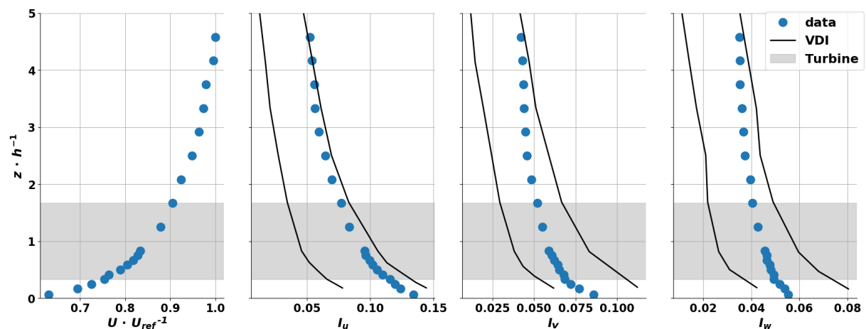
Figure 1: Normalised mean velocity and turbulence intensity profiles of the modelled atmospheric boundary layer. The black lines denote the range of the VDI Guideline's values for slightly rough terrain. The grey area shows the turbine height range. h is the hub height and U_{ref} the reference wind velocity in the wind tunnel.
