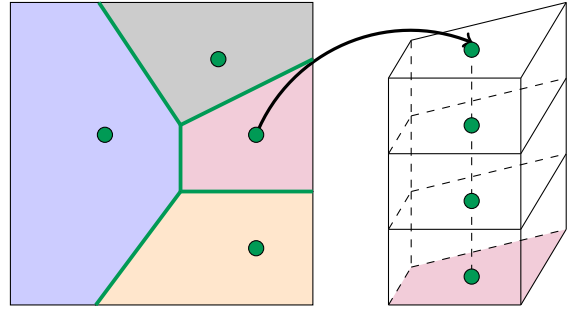
Figure 4: Construction of the Voronoi diagram and 3-dimensional projection.
