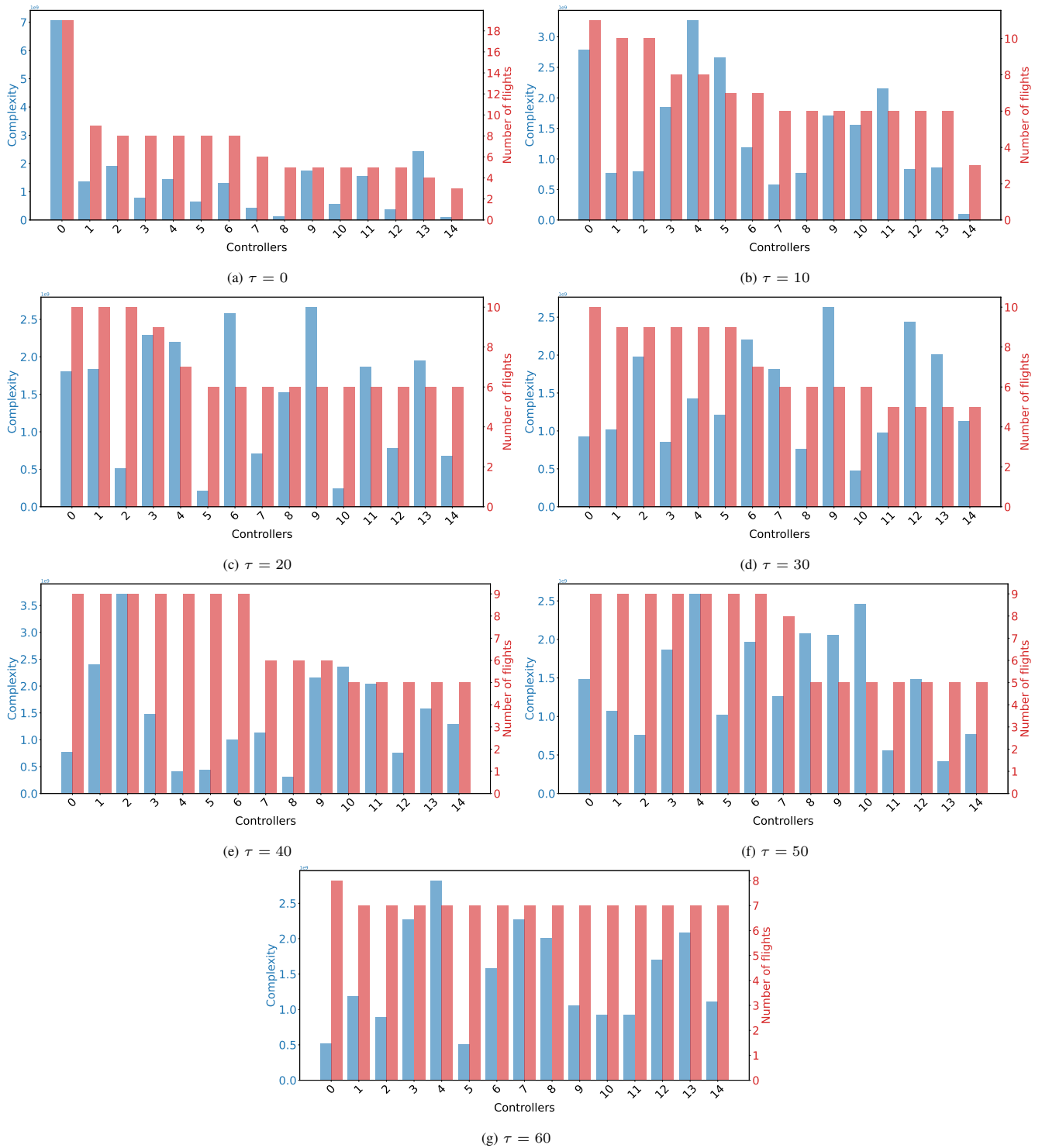
Figure 10. Impact of threshold value \tau on flight volume and complexity per controller (10:20–10:40).
