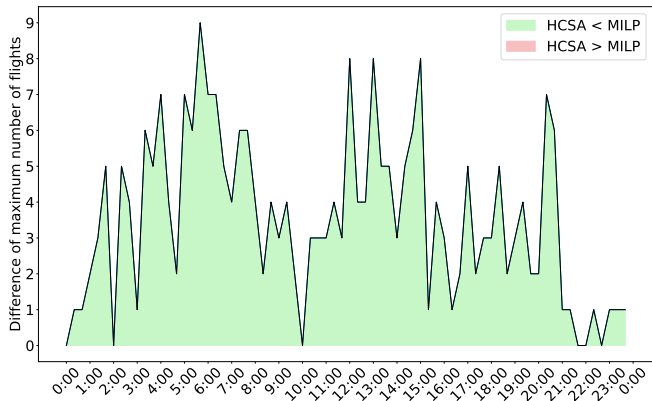
Figure 12. The difference in the maximum number of flights per controller between HCSA and MILP.
