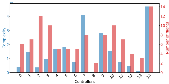
Figure 11. Flight volume and complexity per controller (10:20–10:40) with MILP resolution.
