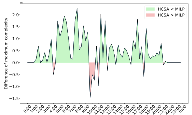
Figure 13. The difference in maximum complexity per controller between HCSA and MILP.
