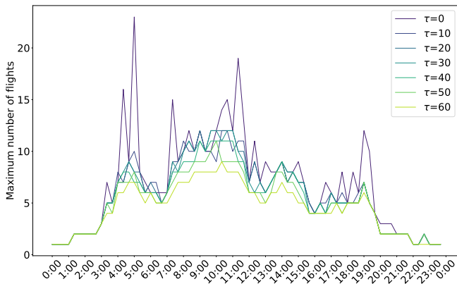
Figure 8. Impact of the threshold value \tau on the number of flights per controller throughout the day.
