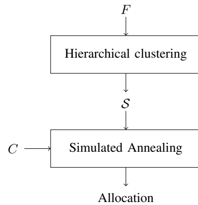
Figure 3. Architecture of the HCSA algorithm.
