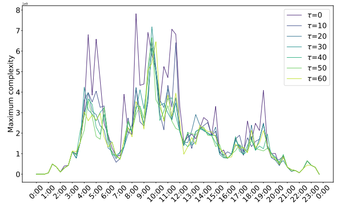
Figure 9. Impact of the threshold value \tau on the number of flights per controller throughout the day.
