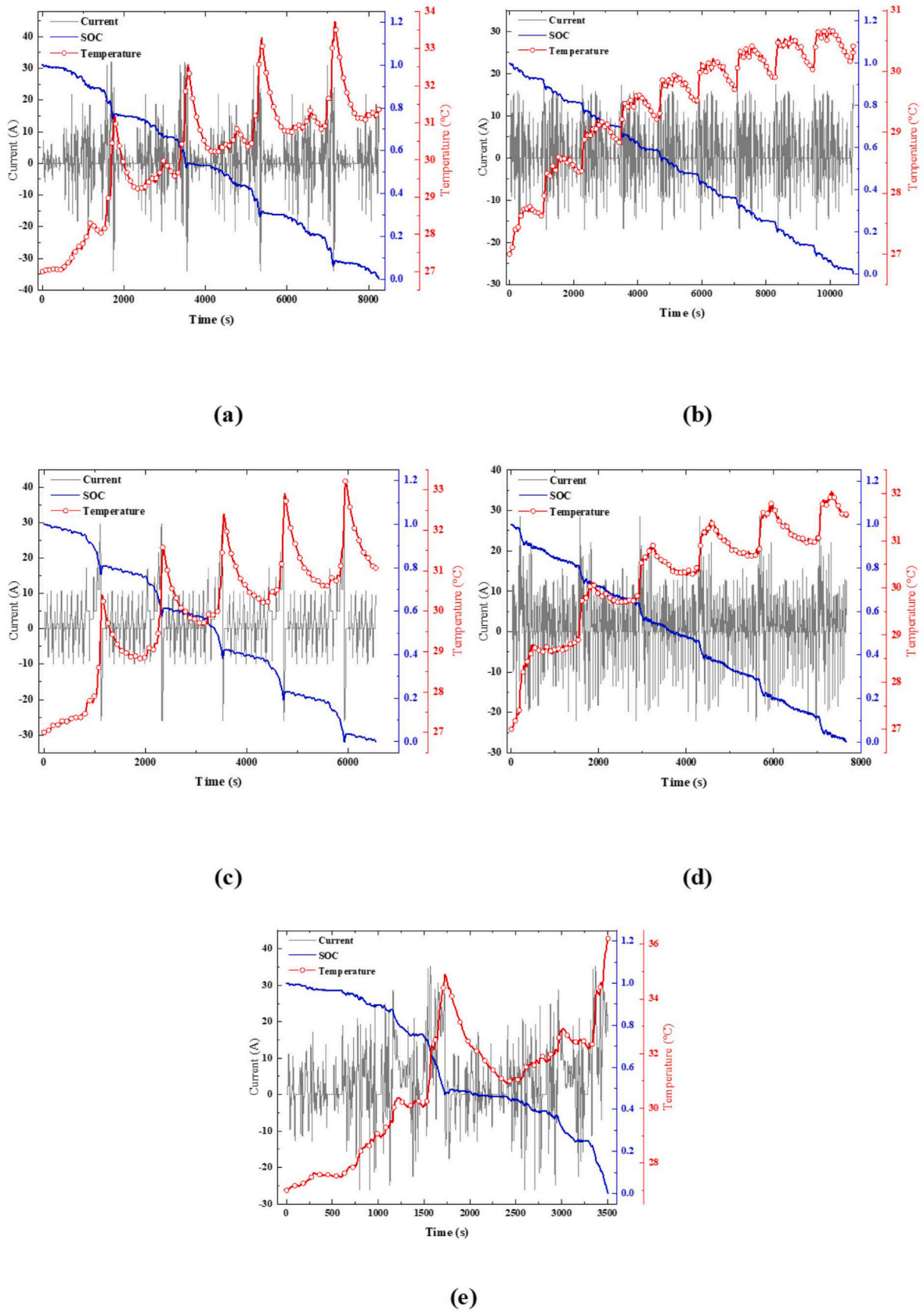
Fig. 15. Cell temperature evolution under realistic discharge current, and cell state of, (a) CLTC, (b) JC08, (c) NEDC, (d) UDSS, (e) WLTP.
