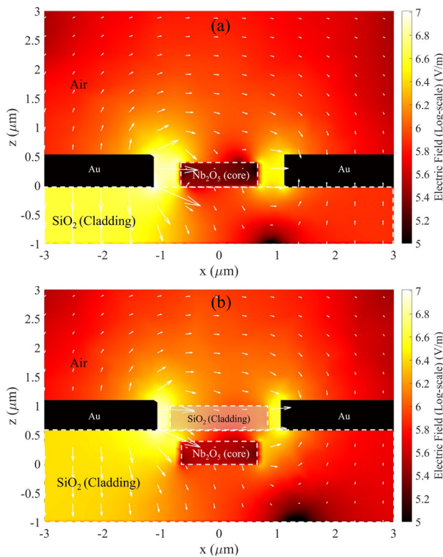
Fig. 11 Log-scale plot of electric field distribution of Strip waveguide a without and b with 600 nm SiO 2 cladding, with white arrows indicating field strength and direction
