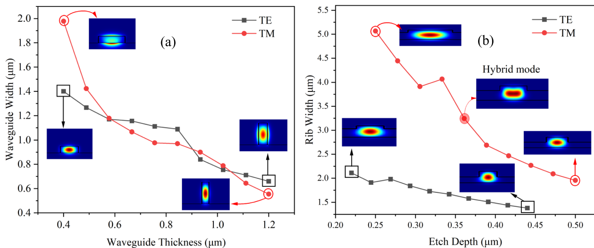
Fig. 2 Single-mode dimension of a strip waveguides, and b rib waveguides, for TE and TM modes. The film thickness used for the rib waveguides is 0.88 μm and 1.0 μm for TE and TM (20–50% etch depth), respectively
