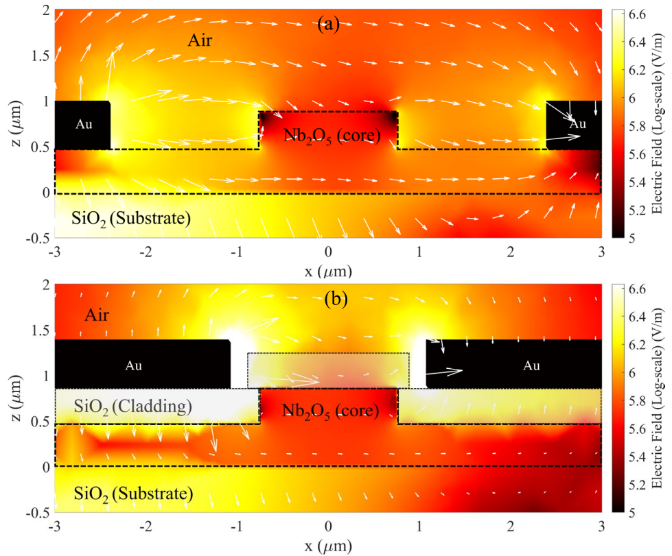
Fig. 10 Log-scale plot of electric field distribution of rib waveguide a without and b with 400 nm SiO 2 cladding, with white arrows indicating field strength and direction
