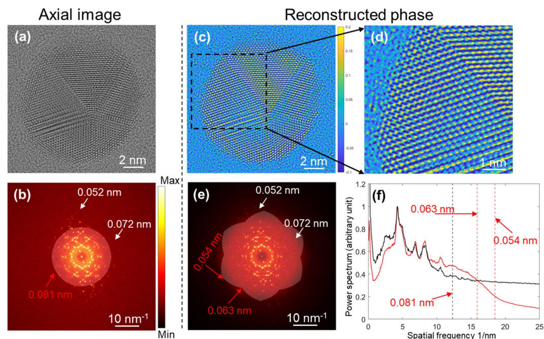
Fig. 3. Phase reconstruction of gold nanoparticles. (a)-(b) Axial TEM image and corresponding power spectrum calculated from the image amplitude. The total fluence is the same as that used for the eFP dataset. In (b), an aperture defined by the axial resolution limit (0.081 nm, where information transfer falls below 10%) is overlaid. (c)-(e) Phase of the reconstructed exit wave and its power spectrum. (d) Enlarged region of (c). In (e), the power spectrum is overlaid with a synthetic aperture using the same 10% information transfer limit and including only spatial frequencies with \geq 2 independent measurements. (f) Circularly averaged power spectra from (b) (black) and (e) (red), respectively. Vertical dashed lines indicate the axial resolution limit in (b) and the synthetic aperture limit in (e). The phase scale bar in (c) is in radians. The intensity of all power spectra is weighted as a power of 0.2 for visualisation of high frequency information and normalized to the strongest reflection at 0.210 nm. For display, phase images in (c) and (d) are gaussian filtered with standard deviation of 4. The tilt magnitude was 12.3 mrad.
