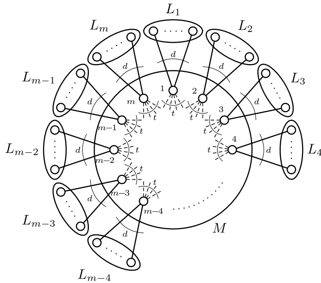
Fig. 12. The unweighted graph G_{m,t,d} of a balanced game \mathcal{G}_{m,t,d} .
