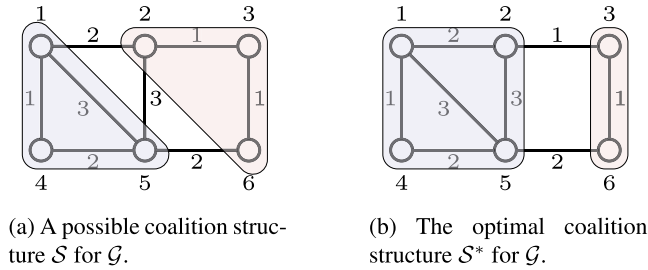
Fig. 5. The instance \mathcal{G} of S-FHG used in Example 2.
