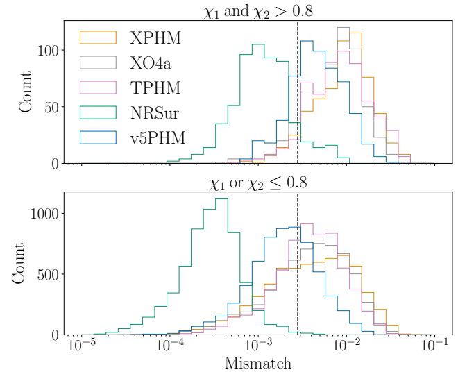
Figure 2. Mismatch accuracy of the waveform models considered in this Letter against 1123 NR simulations at a total mass of 300M_\odot and a range of inclinations between \iota = 0 and \pi/2 . The vertical dashed line at a mismatch of 0.0028 shows the conservative criterion discussed in the text.
