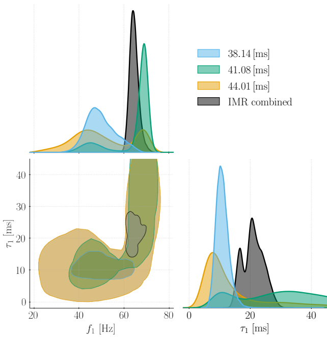
Figure 5. 2D frequency and damping time posterior distribution (90% credible levels), when starting the analysis at late times and assuming a single damped sinusoid with positive frequency; the combined IMR estimates for the longest-lived \ell mn = 220 QNM are shown for comparison. For visualization purposes, we display up to \tau_1 = 45 ms, while the posterior tail extends up to \tau_1 = 80 ms.
