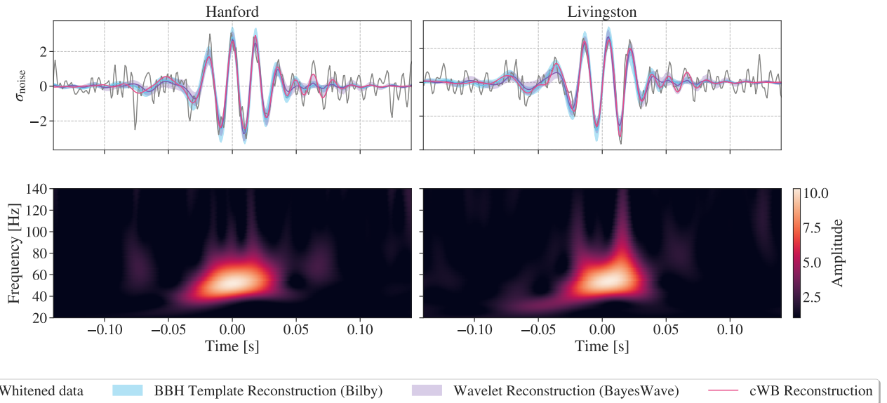
Figure 1. The GW event GW231123 as observed by the LIGO Hanford (left panels) and LIGO Livingston (right panels) detectors. Time is measured relative to 2023 November 23 at 13:54:30.619 UTC. The top panels show the time-domain strain data (black), sampled at 1024 Hz, whitened and then band-pass-filtered with a passband from 20 to 256 Hz (B. P. Abbott et al. 2020). Also shown are the point-estimated whitened waveform from the cWB-BBH search (red), the 90% credible interval of the whitened waveforms inferred from a coherent Bayesian analysis using the combined samples from five BBH waveform models (blue bands), and the 90% credible interval inferred from BayesWave using a generic wavelet-based model (shaded purple). The vertical axis is in units of the noise standard deviation, \sigma_{\text{noise}} . The bottom panels display the corresponding whitened TF representations of the strain data, obtained using a continuous wavelet transform with a Morlet–Gabor wavelet. The color scale is in units of the amplitude of the continuous wavelet transform coefficients.
