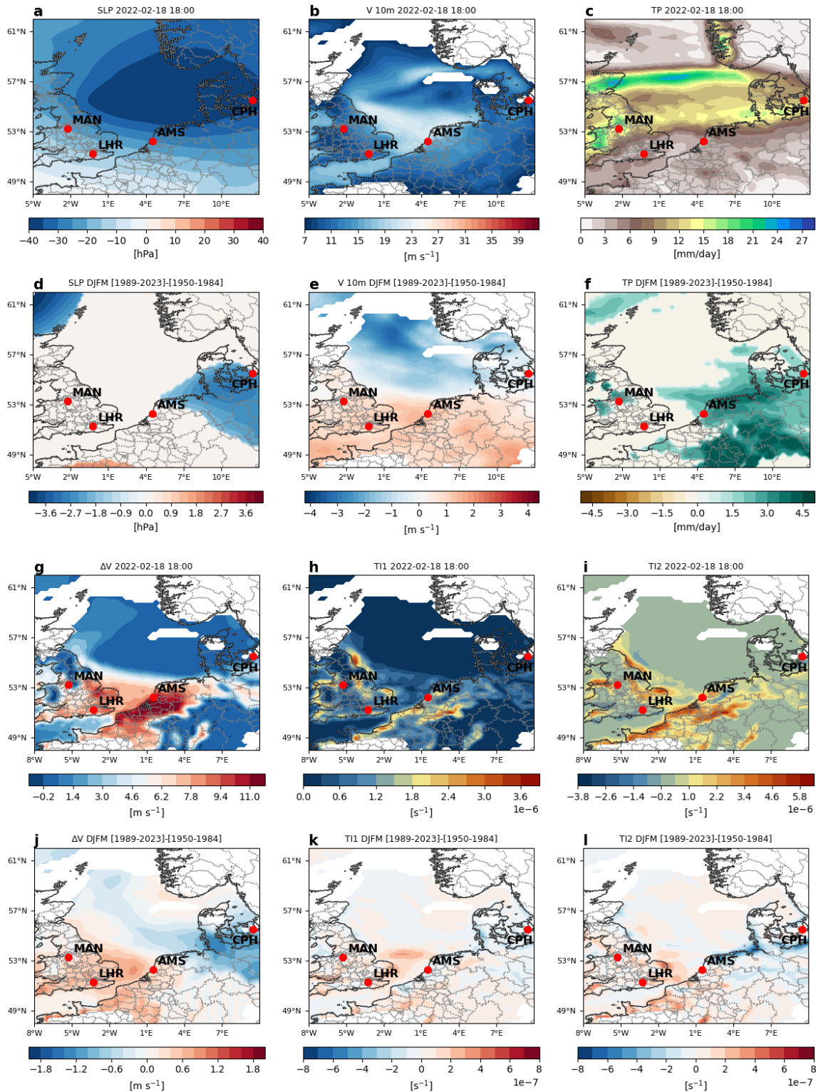
Figure A3. Analogue-based results for the Storm Eunice. SLP (a) anomaly, V 10 m (b), TP (c), \Delta V (g), TI1 (h) and TI2 (i) 12 h after the cyclone time (18 February 2022 18:00). Difference between factual [1989–2023] and counterfactual [1950–1984] period of the average composites at the time-steps corresponding to the analogues for SLP (d) anomalies, V 10 m (e), TP (f), \Delta V (j), TI1 (k) and TI2 (l). In the second row, shadings indicate significant changes.
