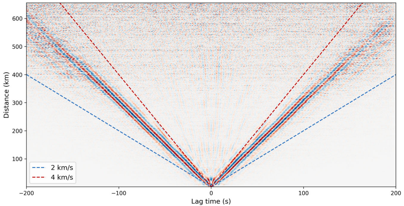
Figure 4. Ambient noise cross correlation using 1 yr of data from the Southern California Earthquake Data Centre: all data are publicly available in the SCEDC AWS cloud storage ( s3://scedc-pds ). The Z-Z component cross-correlation functions are bandpass filtered between 1 and 10 s.
