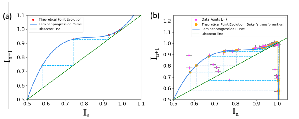
91 Fig. 4. Poincaré maps representing the laminar phase evolution I_{n+1} = f(I_n) : (a) theoretical evolution of a single laminar phase with L = 7 ; (b) 92 theoretical points of 3 successive L = 7 laminar phases considering relaminarization using the baker's transformation. The relaminarization 93 process consists in cutting the blue curve f(x) , taking the upper part, stretching it and folding it back: explaining then the differences between 94 fig (a) and (b). Experimental points for six consecutive cycles of L = 7-8 laminar phases are plotted for comparison.
