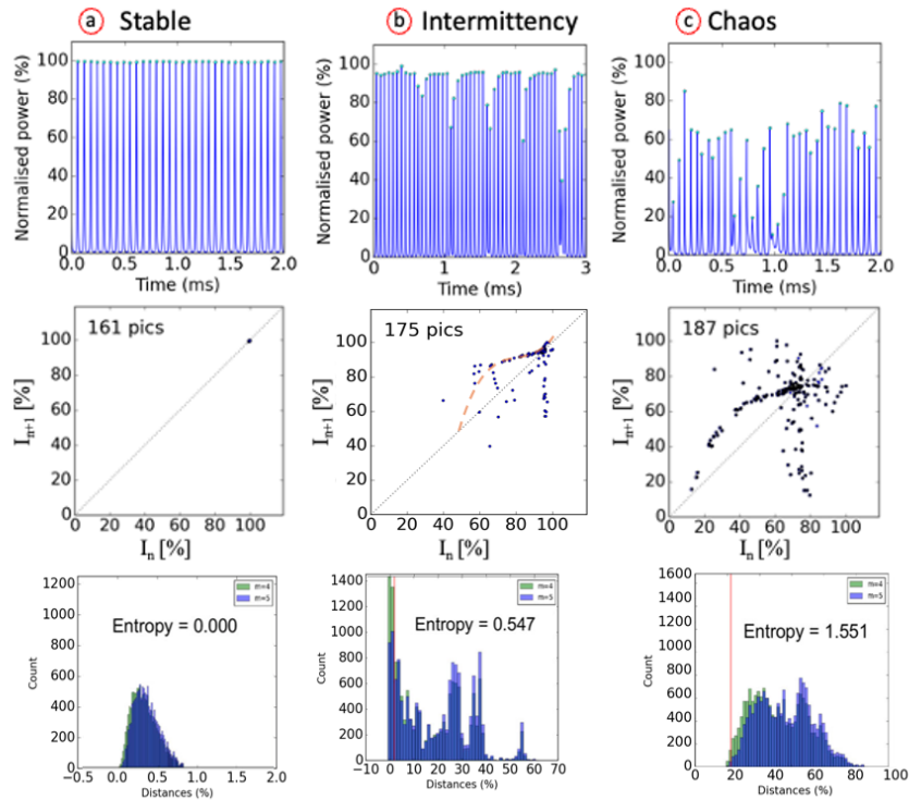
67 Fig. 3. The first line shows the oscillograms, the second line presents the corresponding Poincaré maps of the peak intensities of Q-switched pulses I_{n+1} = f(I_n) , 68 and the third line presents histograms used for calculating the peak entropy (embedded dimension m = 4 and 5). Three different operation regimes are presented: 1 st column 69 (a) corresponds to a stable Q-switched regime, 2 nd column: (b) corresponds to an intermittency regime, 3 rd column (c) corresponds to a chaotic regime.
