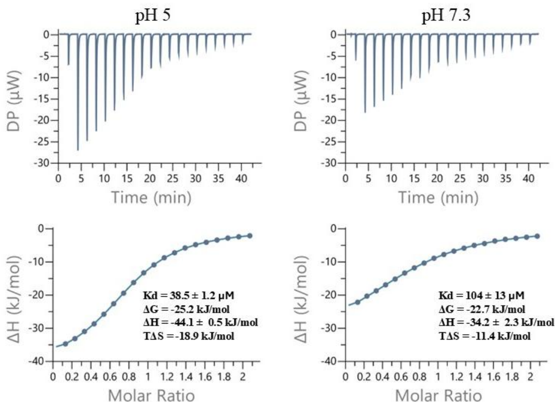
Figure 5. Titration of galactose into LecA solution by ITC at two different pH. Top: data obtained from 20 automatic injections, 2 \mu L each, of Gal (3 mM) into the cell containing LecA (0.3 mM). Lower: plot of the total heat released as a function of total ligand concentration for the titration shown above. The solid line represents the best least-squares fit for the obtained data.
