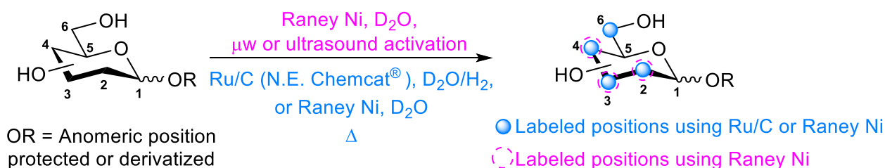
Scheme 1. State-of-the-art work using metal-mediated HIE for the labeling of carbohydrates
