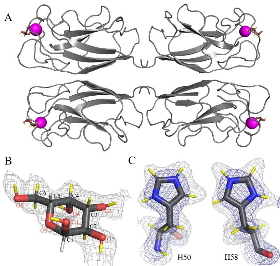
Figure 2. Joint X-ray/neutron crystal structure of D-LecA/Gal-d 10 complex. (A) Simplified representation of one tetramer (chains A-D) with calcium ions represented as magenta spheres and galactose molecules as sticks (B) Neutron scattering-length density map shown as grey mesh ( 2mF_o-DF_c contoured at 1.0\sigma ) around the galactose ligand with deuterium atoms colored yellow and hydrogen atoms (at C1 and C5) colored white. (C) Neutron scattering-length density map in grey ( 2mF_o-DF_c contoured at 1.0\sigma ) and X-ray electron density map in blue ( 2mF_o-DF_c contoured at 1.4\sigma ) for charged histidine residues, His50 and His58, of chain A.
