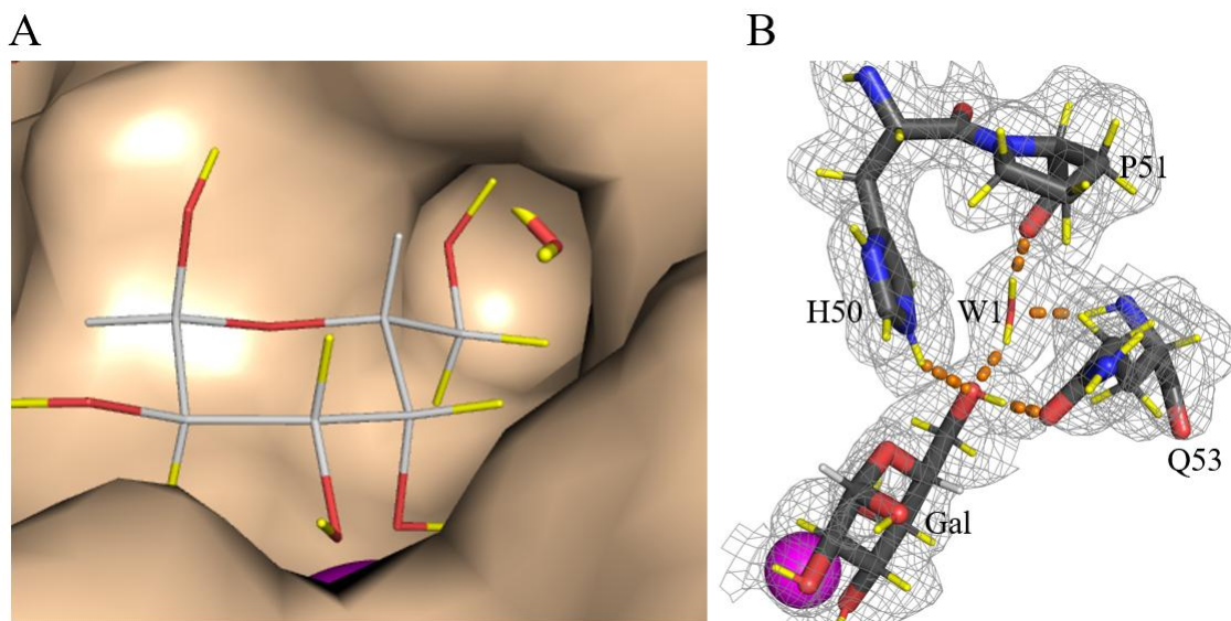
Figure 4. Conserved water molecule W1 in the neutron structure of the D-LecA/Gal-d 10 complex. (A) Protein surface representation of the binding pocket. (B) Hydrogen-bond network around W1 with the 2mF o -DF c neutron density map (grey mesh) contoured at 0.8σ.
