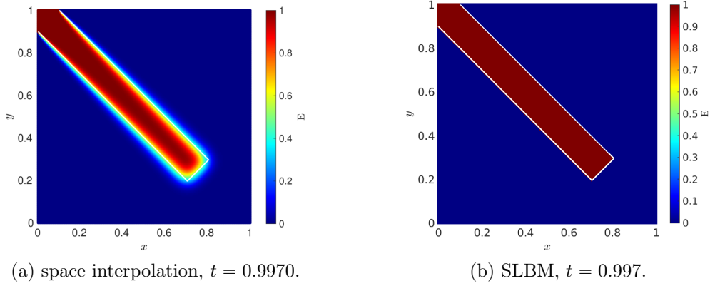
Figure 11: Evolution of the total energy E for the second case with the space interpolation approach at t = 0.9970 in (a) and with the SLBM approach at t = 0.9970 in (b). The exactly streamed beam is represented by a white contour in (a) and (b).
