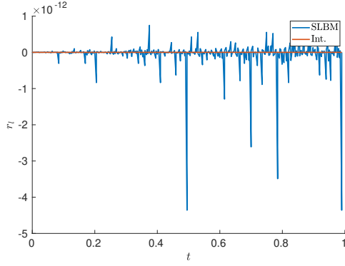
Figure 9: Evolution of the energy residual for the first case with the SLBM approach in blue and the space interpolation in red.
