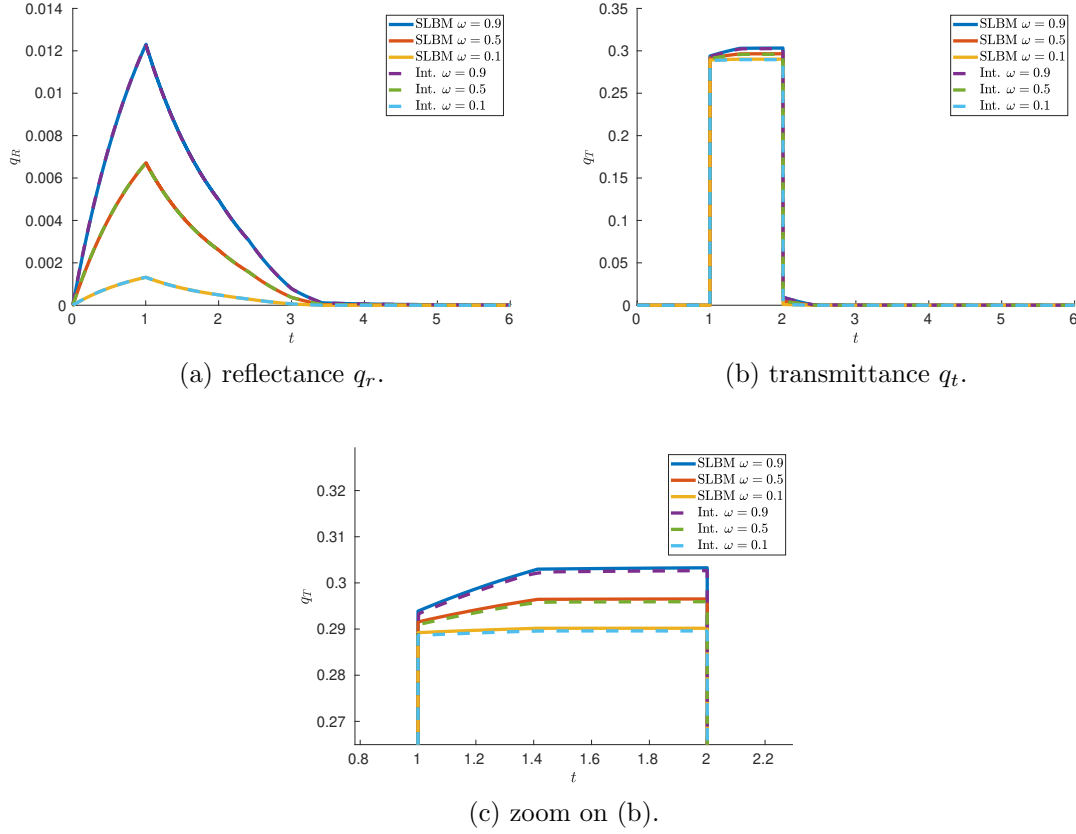
Figure 15: Evolution of the reflectance q_r in (a) and transmittance q_t in (b) with a zoom on the upper part in (c), computed with the SLBM and interpolation approaches with different albedo values: \omega = 0.9, 0.5 and 0.1 .
