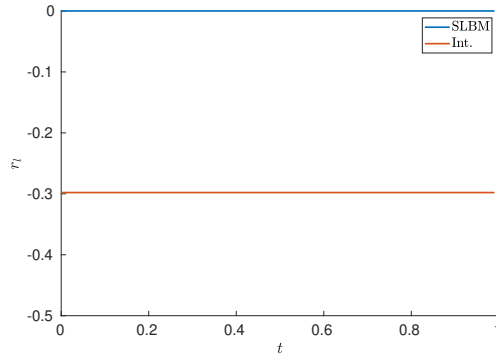
Figure 12: Evolution of the energy residual for the second case with the SLBM approach in blue and the space interpolation in red.
