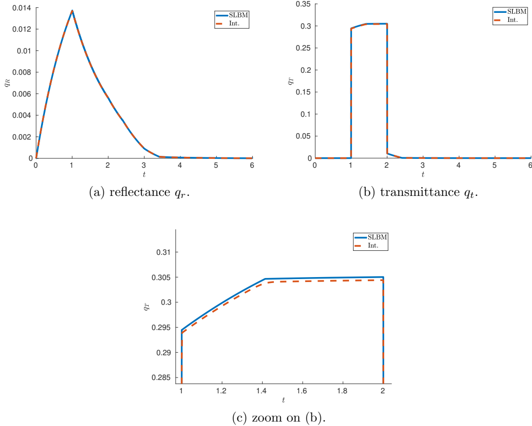
Figure 14: Evolution of the reflectance q_r in (a) and transmittance q_t in (b) with a zoom on the upper part in (c), computed with the SLBM and space interpolation approaches with an albedo \omega = 1.0 .
