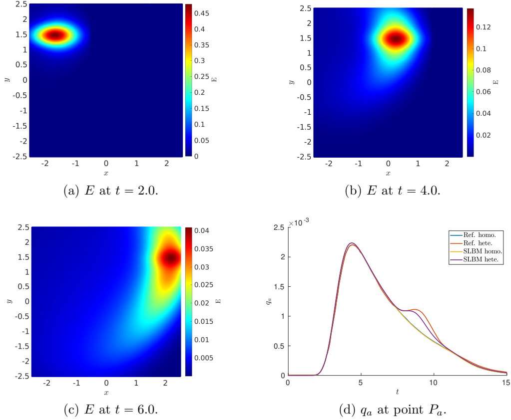
Figure 17: Evolution of the total energy E at t = 2.0 in (a), 4.0 in (b) and 6.0 in (c) for the heterogeneous medium case. Evolutions of the back-scattered flux q_a at point P_a for the homogeneous and heterogeneous medium cases one as well as those obtained in [27], used as reference.
