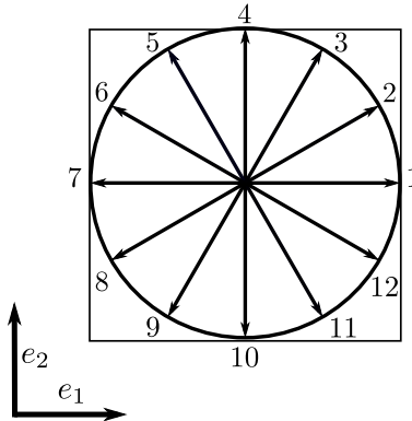
Figure 3: Example of a uniformly spaced direction set used in [45] in the case where d = 2 , N = 12 and \Delta x = v\Delta t .
