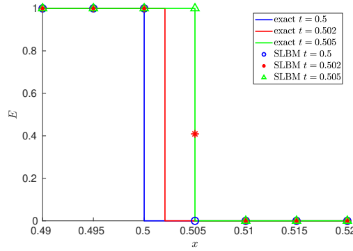
Figure 10: Evolution of the exact total energy E and the one obtained with the SLBM approach, for the first case, at nodes of \mathcal{L}_x belonging to the segment [0.49, 0.52] \times \{0\} at t = 0.50 , t = 0.502 and t = 0.505 .
