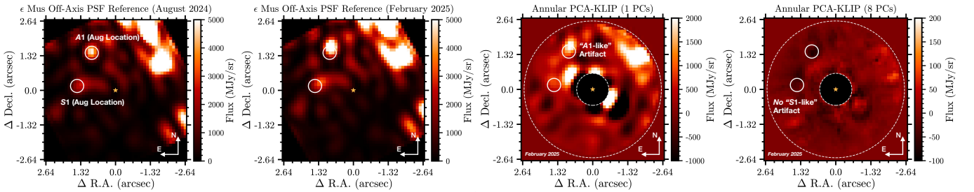
Figure 16. Left: the de-rotated off-axis \epsilon Mus reference for \alpha Cen B for the 2024 August observations. It acts as a proxy for and shows the diffraction features expected from \alpha Cen B in vicinity of \alpha Cen A. The locations of the detections of S1 and A1 in 2024 August are marked. Center left: the de-rotated off-axis \epsilon Mus reference for \alpha Cen B for the 2025 February observations. The diffraction pattern is nearly identical to that observed in 2024 August. Center right: joint PCA-KLIP reduction of the 2025 February data set with one PC showing the presence of an “A1-like” artifact. Right: joint PCA-KLIP reduction with eight PCs showing that no persistent artifacts are seen at the location of S1 (and A1).
