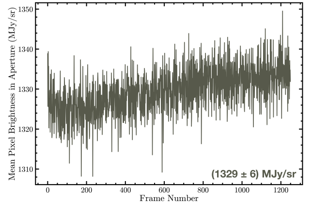
Figure 10. The average pixel brightness in a 3 pixel radius aperture centered on S1 in the background-subtracted Stage 2b \alpha Cen AB integrations from 2024 August. The time series does not show any sharp transitions (increases) that would appear as an artifact at the location of S1 after PSF subtraction.
