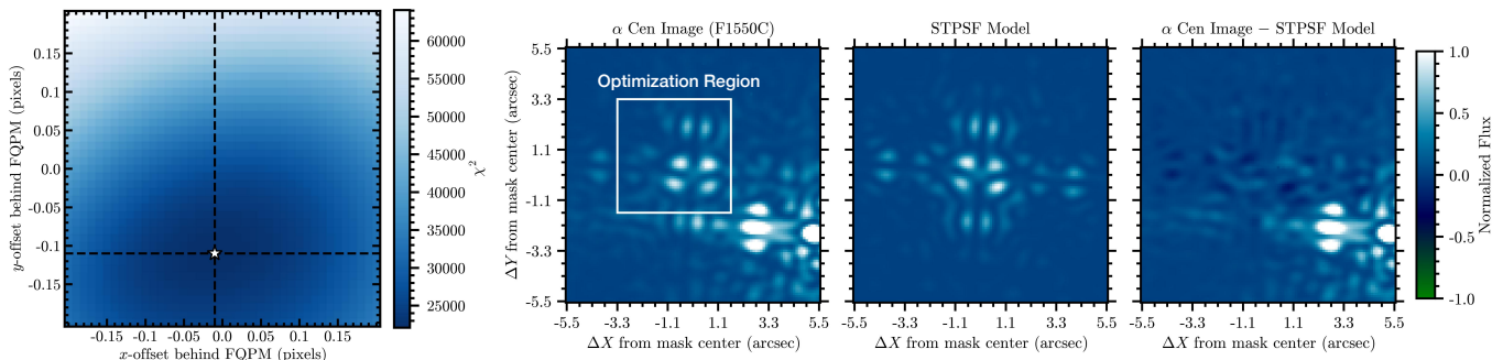
Figure 2. Example determination of stellar position behind the MIRI 4QPM for \alpha Cen A in the 2024 August observation. Left: \chi^2 map obtained after subtracting STPSF models generated by varying the stellar position behind the mask (marginalized over the model PSF flux scale factor parameter). The best-fitting PSF (minimum \chi^2 ) is marked with a white star. Right: from left to right, the observed \alpha Cen A PSF, best-fitting STPSF model, and residual image after taking the difference are shown. The white box designates the region over which \chi^2 was minimized.
