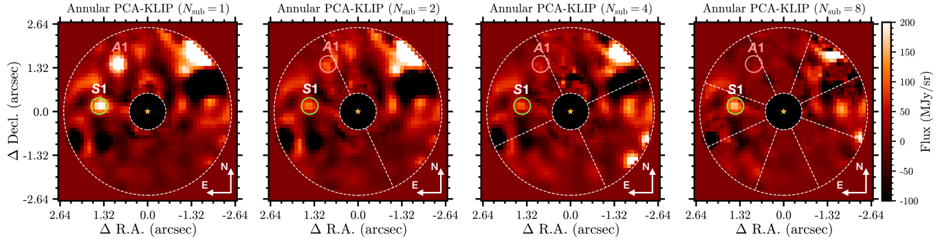
Figure 8. Joint PCA-KLIP subtraction of \alpha Cen AB for the 2024 August observations for different number of azimuthal subsections ( N_{\text{sub}} ). S1 is recovered in all reductions, whereas A1's signal disappears as N_{\text{sub}} increases.
