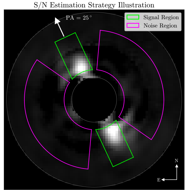
Figure 20. Illustration of how the S/N map is generated for the detection of extended emission. The figure shows an example of a signal region (green) at one PA, along with the corresponding perpendicular annular noise region (purple), using the coplanar asteroid belt analog (ABA) ABA-1 exozodi model injected into the April data. The S/N is calculated by varying the aperture’s PA and length.
