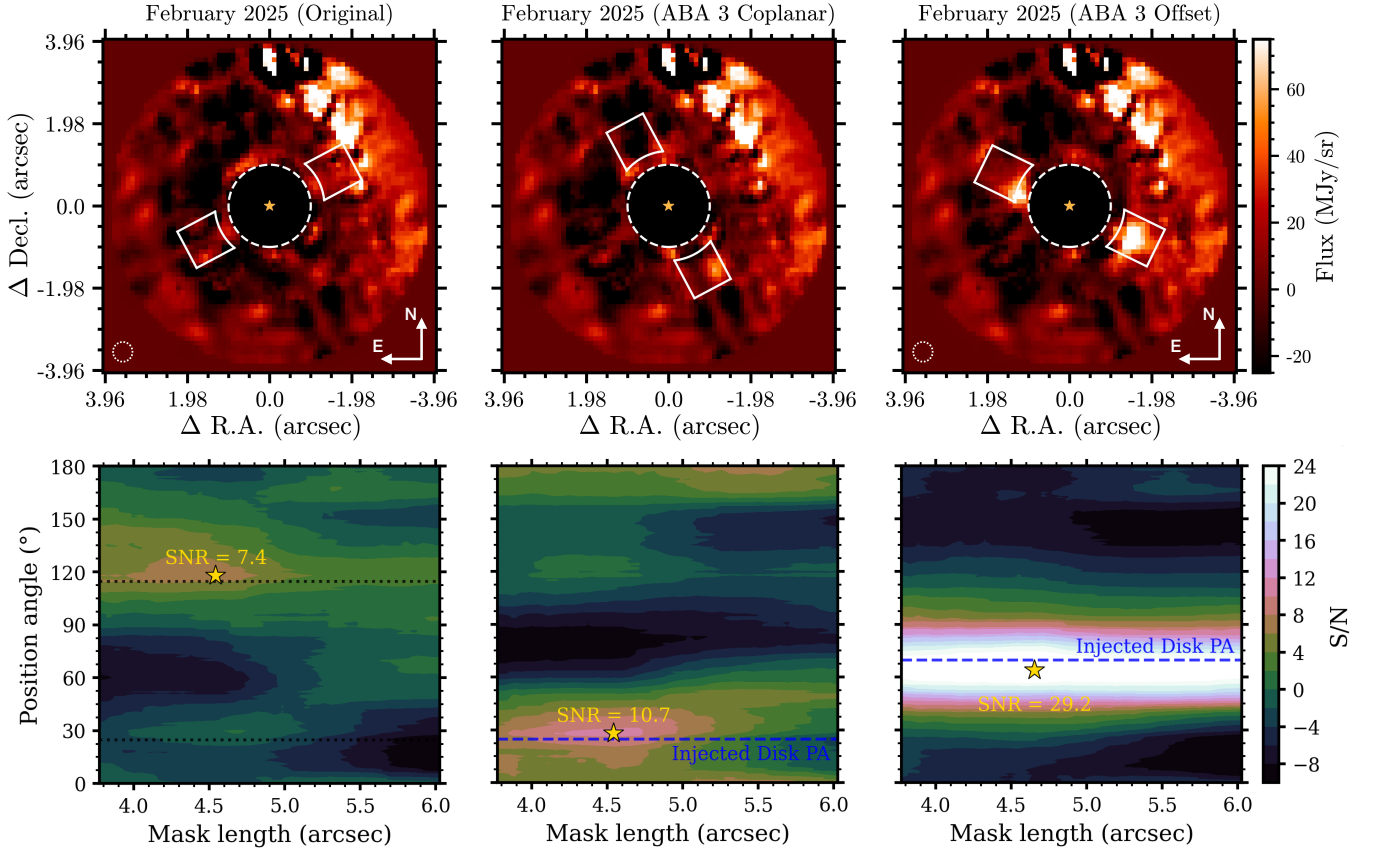
Figure 21. PSF-subtracted images (top) and the corresponding extended emission S/N maps (bottom) for the 2025 February observation for three cases: (left) original data, (center) ABA-3 exozodi model injected with a coplanar orientation, and (right) ABA-3 exozodi model injected with an offset orientation. In the image plots, a one FWHM diameter beam is indicated in the bottom left corner with a dotted circle. The aperture that yields the highest S/N (marked by a star in the S/N maps) is shown in the images. For the original data, dotted lines in the S/N map mark the PAs of the 4QPM transition boundaries. For the injected cases, dashed lines mark the PAs of the injected disks.
