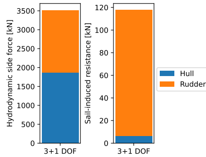
Figure 4: Forces distribution at s = 2 for the KVLCC2 at V = 15.5 kt.
