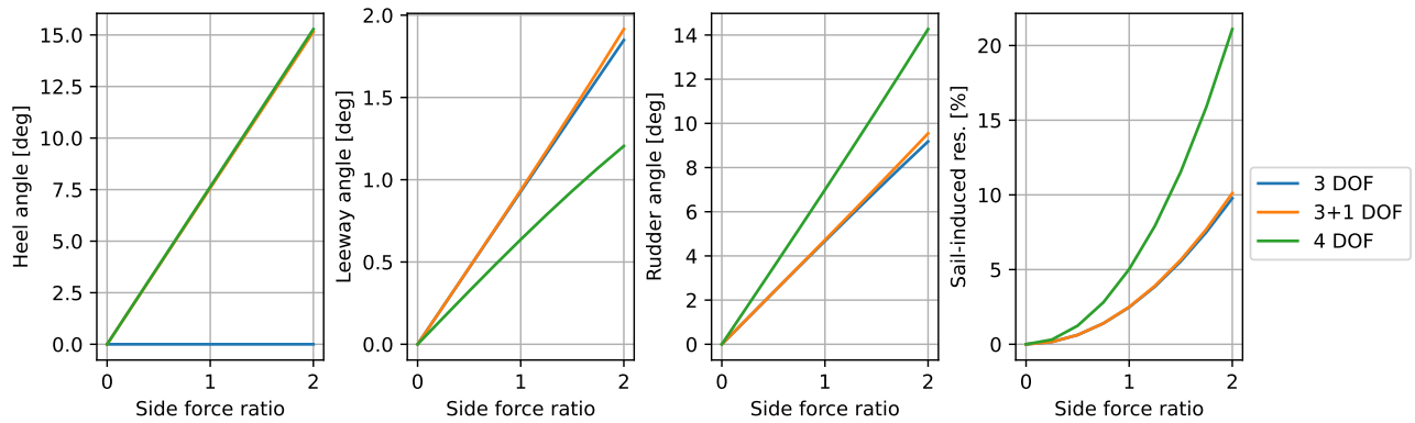
Figure 5: KCS response to an increasing aerodynamic side force at V = 20 kts.
