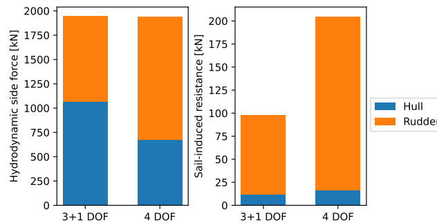
Figure 6: Forces distribution at s = 2 for the KCS at V = 20 kt.
