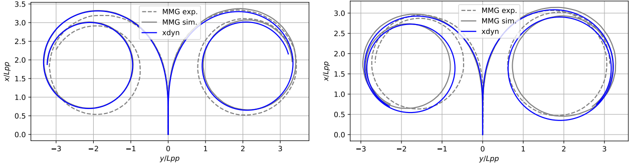
(a) KVLCC2 at scale 1/45.7 with an initial speed u_0 = 1.180 m/s (3 DOF).
