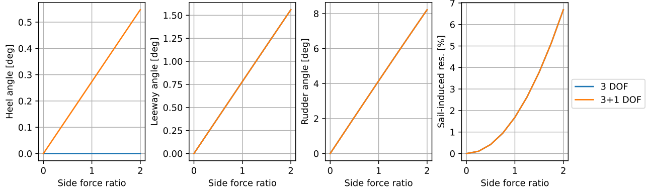
Figure 3: KVLCC2 response to an increasing aerodynamic side force at V = 15.5 kt.
