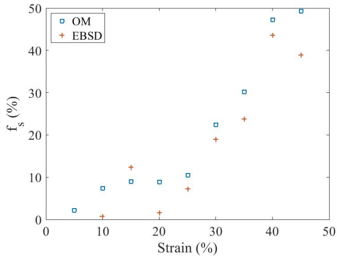
Figure 5: Martensitic phase fractions measured from optical microscopy and SEM - EBSD observations (all non austenitic phases)
