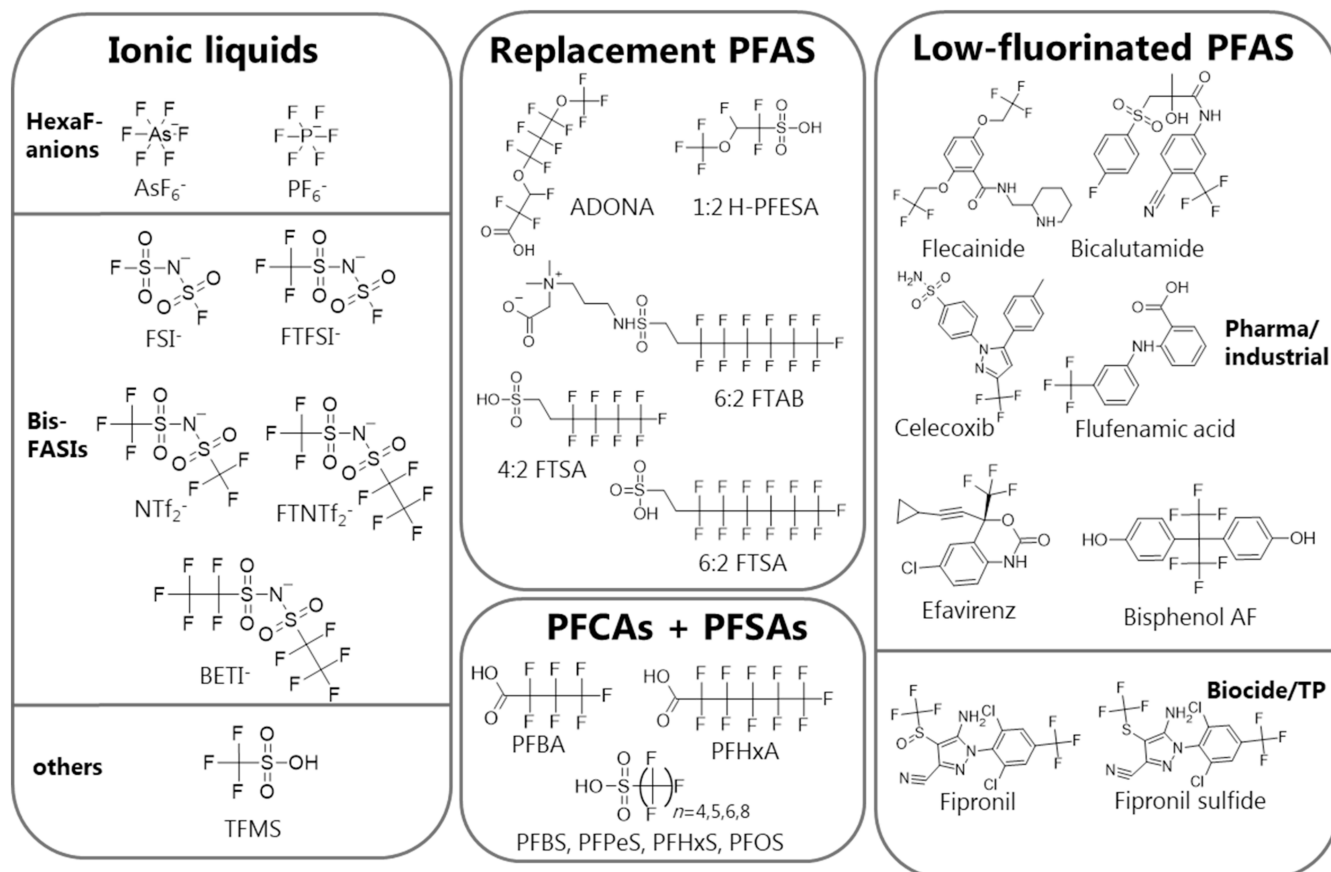
Figure 2. Chemical structures of PFAS and inorganic fluorinated compounds identified in European wastewater effluent samples, available as the SFCPFASFIONS list. 48
