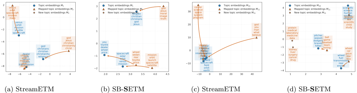
Figure 4: PCA projections of topic embeddings (at timesteps t = 1-2 for (a)-(b), and t = 11-12 for (c)-(d)). Arrows indicate associations between topics across consecutive timesteps. In (c), the topics in blue are: god/jesus/interpretation/moral/belief, space/spaceship/field/orbit/earth, dealer/engine/driver/rear/ford.
