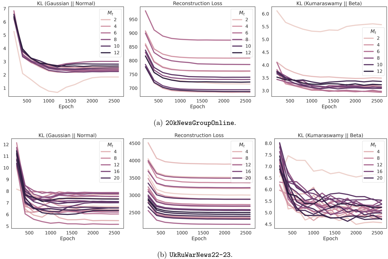
Figure 8: Losses evolution during training. SB-SETM (COT-based merging strategy and K_{init} = 50 ).
