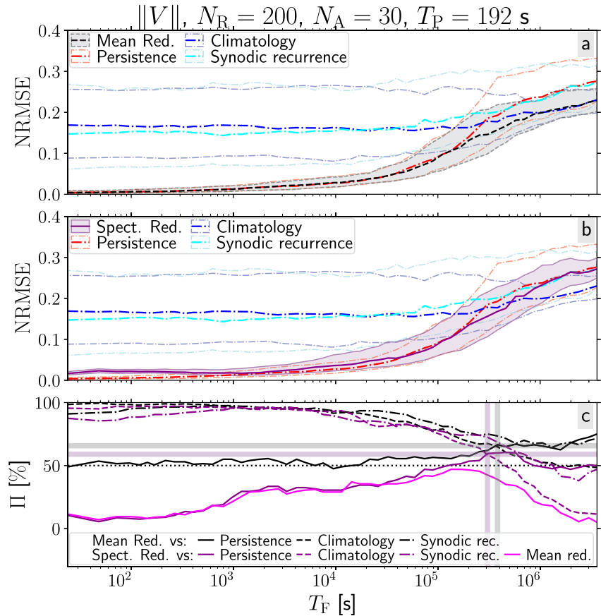
Figure 8. Performance of mean-reduced (black, panels a and c) and spectral-reduced (purple, panels b and c) forecasts of proton velocity magnitude as a function of the size of the forecast, T_F . Results are shown for N_A = 30 individuals, N_R = 200 reference times and a pattern size T_p = 192 s. Panels (a, b): Median and quartiles (lighter) of NRMSE. Comparison with the persistence (red dash-dotted), the climatology (blue dash-dotted), and the synodic recurrence (cyan dash-dotted). Panel c: Proportion of positive Skill relative to persistence (straight), to climatology (dashed), and to synodic recurrence (dash-dotted), and of spectral-reduced relative to mean-reduced forecasts (magenta). The crosses indicate the predictability \Pi = N_R (Skill > 0) where \Pi_{\text{persistence}} = \Pi_{\text{climatology}} and the associated optimal lead time T_L for mean-reduced (gray) and spectral-reduced (pink) forecasts.
