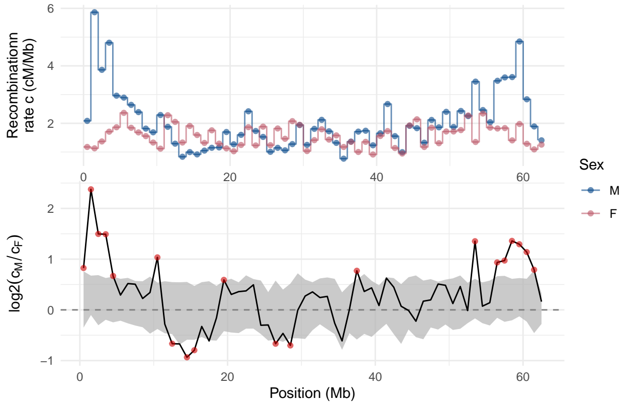
Recombination map on chromosome 24
