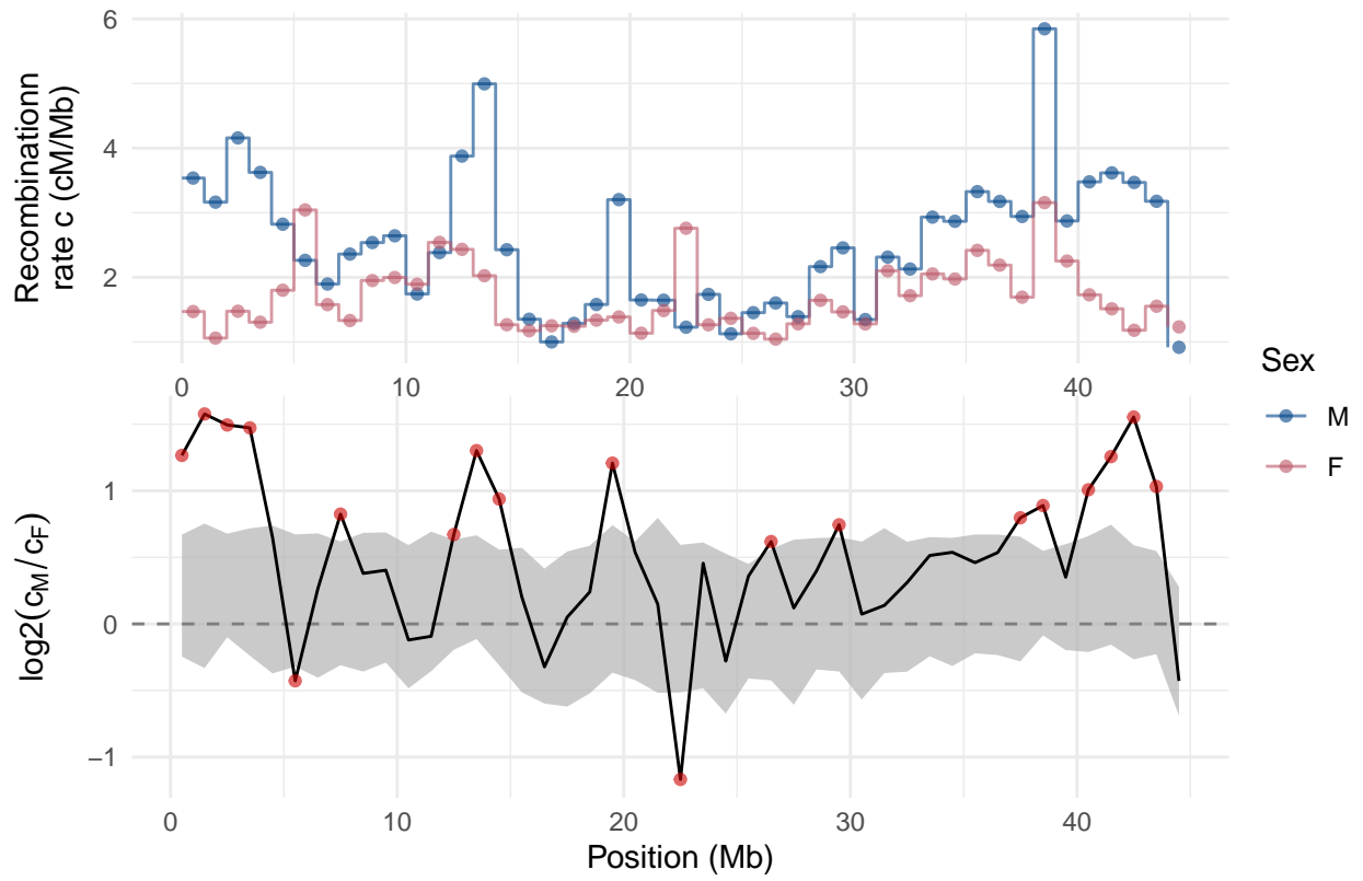
Recombination map on chromosome 28
