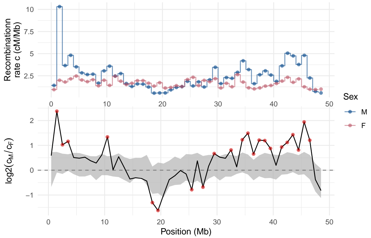
Recombination map on chromosome 23
