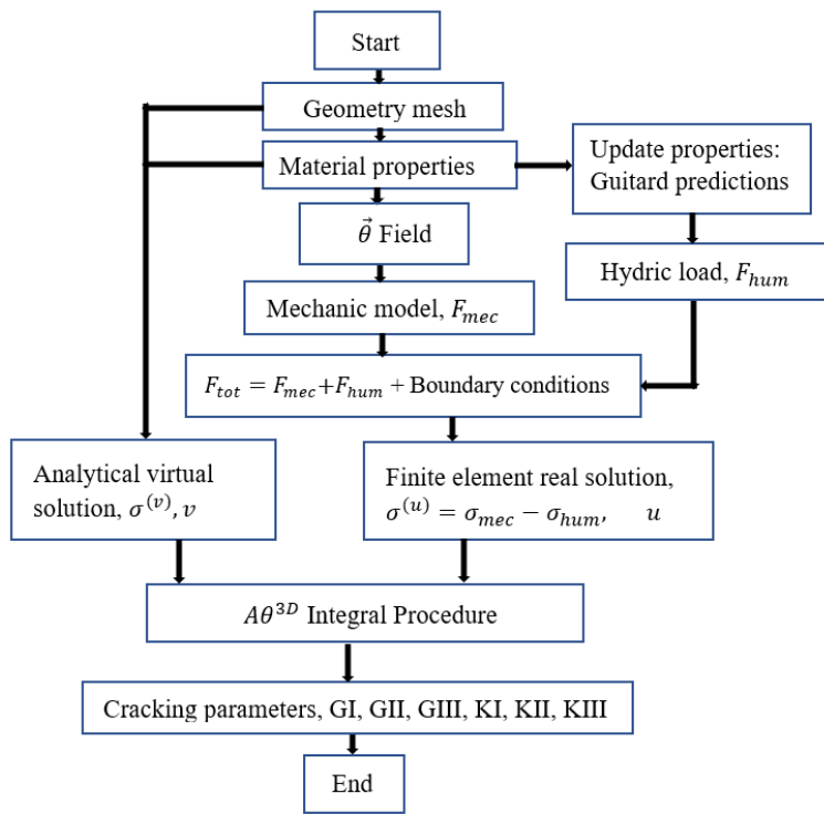
Figure 3: Finite element numerical scheme implementation.
