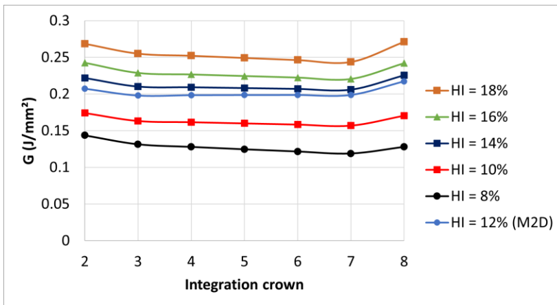
Figure 4a: Path independence verification of energy release rate for 8% to 18% moisture content.
