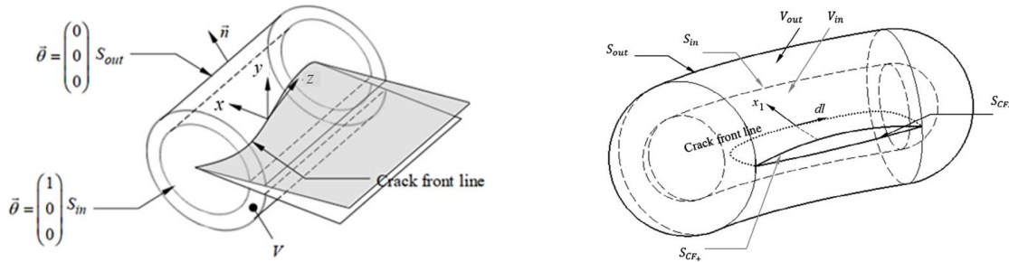
Figure 1: \theta field in 3D (left), Integration domain (right).
