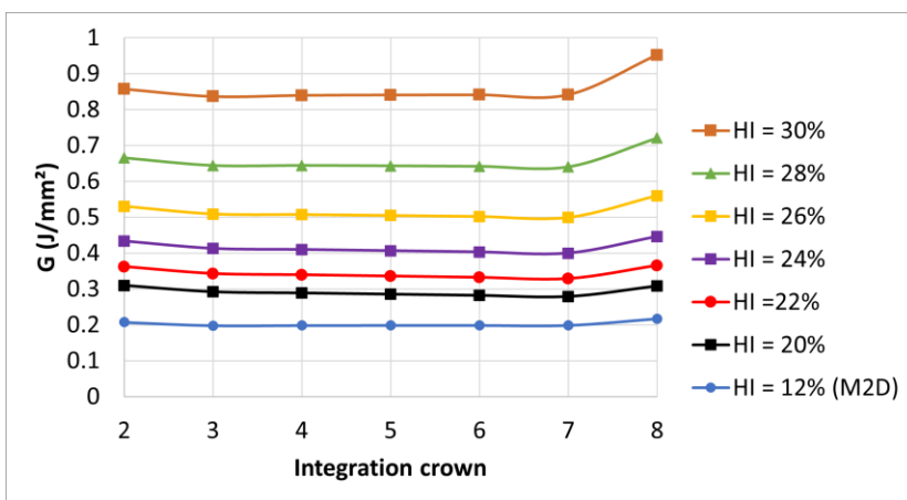
Figure 4b: Path independence verification of energy release rate for 20% to 30% moisture content.
