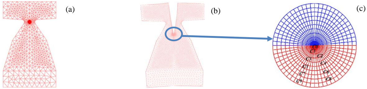
Figure 2: (a) MMCG mesh, (b) Opening mode, (c) Radiating mesh at the crack tip.
