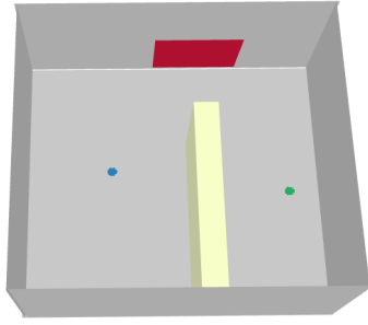
Fig. 2: Simulated environment composed of square room, one transmitter, one receiver, one RIS, and one obstacle.
