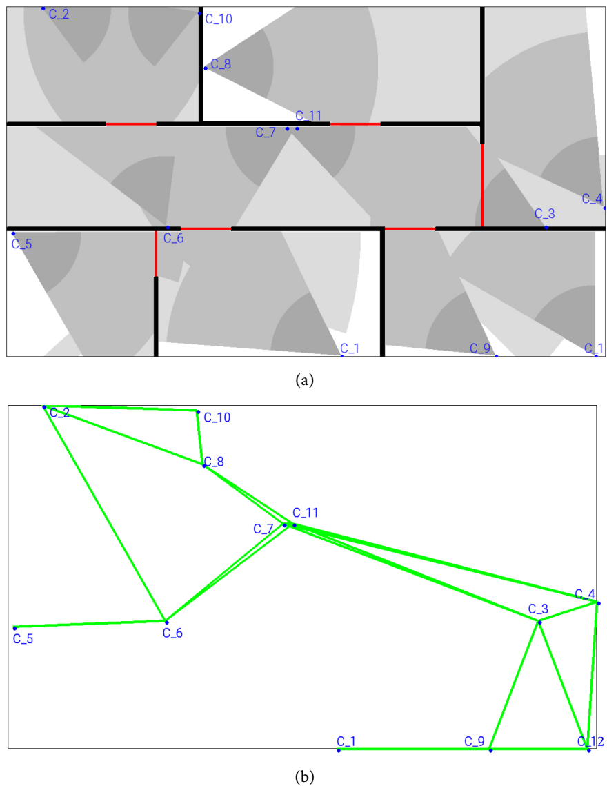
Figure 13. Deployment and connectivity of 12 cameras in the indoor scene. (a) Deployment of 12 cameras in an indoor scene, (b) Resulting connectivity with 12 cameras.
