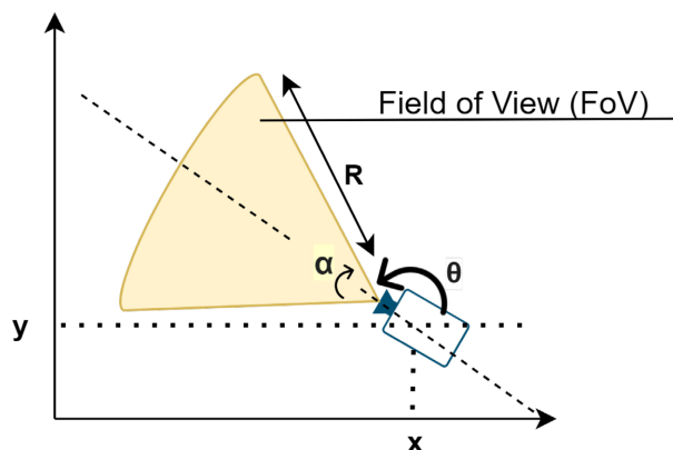
Figure 1. Camera's parameter.
