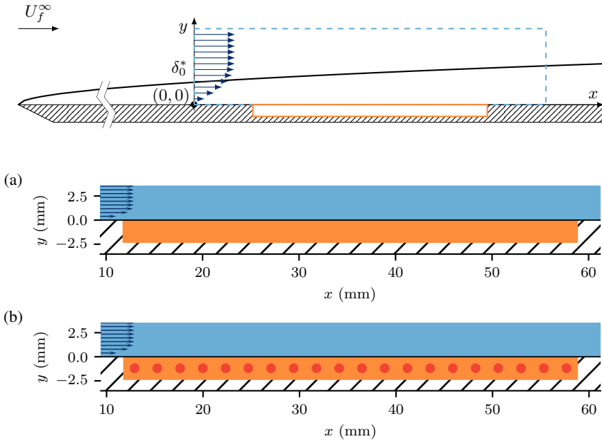
Figure 1. Wall-mounted compliant wall (orange) in a zero-pressure-gradient boundary-layer flow in water (blue). The origin of the frame of reference is positioned at the beginning of the computational domain: x and y indicate respectively the streamwise and wall-normal coordinates. The leading edge of the plate (i.e., the origin of the boundary layer) is positioned at x \approx -47.7 cm, for a uniform free-stream velocity U_f^\infty = 10 m/s. The resulting Reynolds number based on the displacement thickness at the inflow ( \delta_0^* ) is Re_{\delta_0^*} = 3000 . (a) shows the conventional set-up from Pfister et al. (2022) with a compliant structure made by an homogeneous viscoelastic material, while (b) depicts the phononic compliant surface obtained by introducing stiffer inclusions (in red) within the homogeneous matrix and subject of the current study.
