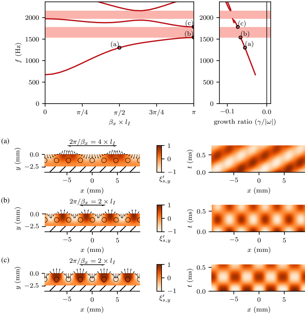
Figure 7. (Top) Dispersion relation from Bloch analysis for an isolated, x -periodic phononic medium. The shaded red areas highlight the bands of angular frequencies for which no eigenvalues are found (band-gaps). (a-c) report the time-space evolution of the modes labelled in the top figures. On the left, the colour map reports the vertical displacement field in the solid domain at t = 0 , while the vectors the displacement at the interface. On the right, the colour map reports time-space evolution of the vertical displacement at the interface over one oscillation.
