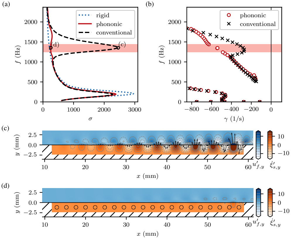
Figure 2. Global, coupled, linear stability analyses of the conventional and phononic compliant surfaces in Figure 1 interacting with a laminar boundary-layer flow. The optimal, harmonic, forced response (a) and eigenvalue analysis (b) are reported for the conventional compliant surface (black, dashed line and crosses) and the phononic one (red, solid line and white-filled, red circles), respectively. The blue dotted line in (a) indicates the response over a rigid wall. The spatial structure of the response of the fluid-structural system at the TWF amplification peak ( f \approx 1350 Hz) is reported both for the conventional (c) and phononic (d) compliant surface. The colour indicates the real part of the vertical velocity in the fluid (blue) and solid (orange) phases, while the black vectors the real part of the surface displacement at the interface. The red shaded area in (a) and (b) indicates the identified band-gap of the phononic surface ( 1241 \text{ Hz} \leq f \leq 1439 \text{ Hz} ), encompassing the two truncation modes (see Figure 3).
