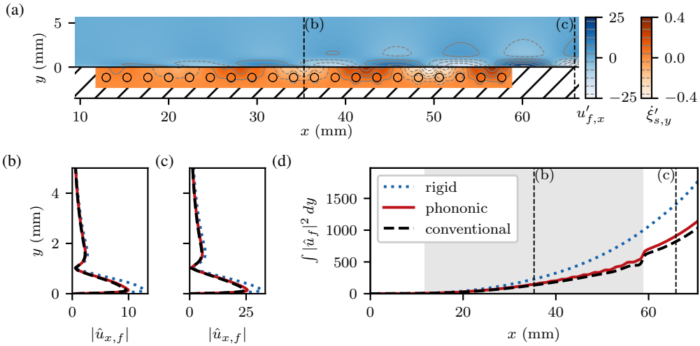
Figure 4. Spatial attenuation of TSW. (a) depicts the perturbation fields over the phononic surface for the optimal, harmonic, forced response at the amplification peak of TSW, f = 210 Hz in Figure 2. The colour shows the streamwise component of the perturbation velocity in the fluid ( u'_{f,x} , in blue) and the vertical component of the solid velocity ( \xi'_{s,y} , in orange). (b) and (c) report the magnitude of the streamwise velocity perturbation field at x = 35 mm and x = 66 mm. The dotted, dashed, and solid curves indicate respectively the rigid, conventional compliant, and the phononic compliant surfaces. (b) reports the velocity perturbation in the fluid phase; the gray area indicates the streamwise extent of both the conventional and the phononic compliant walls.
