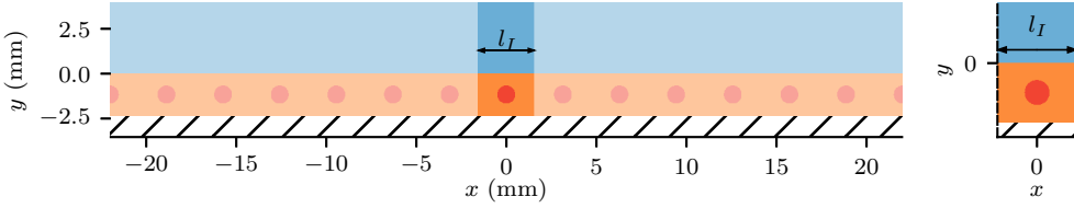
Figure 6. Infinite, periodic, phononic surface interacting with a fluid at rest. The periodic cell (right) – clamped at the bottom and interacting with the fluid at the top – with span l_I is periodically and infinitely replicated along the x -direction (left).
