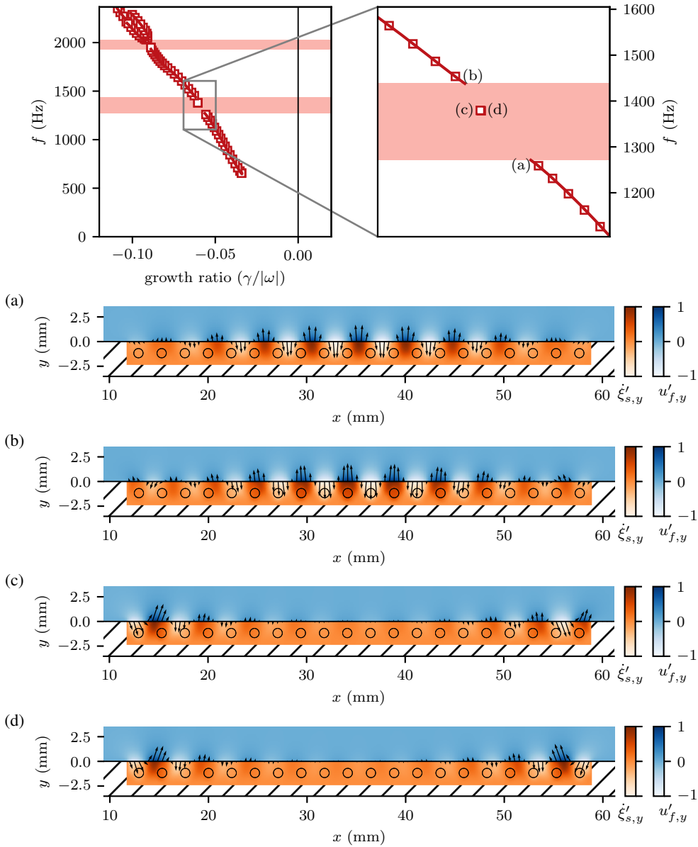
Figure 10. Comparison between the fluid-structural eigenvalues branches computed by means of the Bloch analysis (lines, see Figure 8) and the eigenvalues of the finite-length surface (squares). A fluid at rest is considered for the two analyses. The coloured shaded areas indicate the band-gaps predicted by the Bloch analysis. (a-d) report the respective modal shapes of the modes labelled in the top figure (for a finite-length structure).
