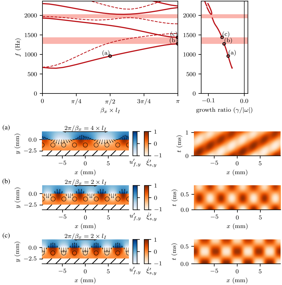
Figure 8. Dispersion relation from the Bloch’s analysis for a viscoelastic, periodic solid interacting with a fluid at rest (solid lines). The shaded areas highlight the bands of frequencies for which no eigenvalues are found (band-gaps). The dashes lines report the dispersion relation for the isolated periodic solid (see Figure 7). (a-c) report the modal shapes of the modes labelled in the top figure. On the left, the colour maps report the vertical displacement field in the solid (orange) and fluid (blue) domains at t = 0 , while the vectors the displacement at the interface. On the right, the time-space evolution of the vertical displacement at the interface is reported over one oscillation.
