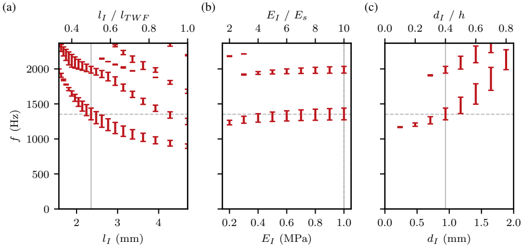
Figure 9. Parametric study on the spacing ( l_I , a), Young modulus ( E_I , b), and diameter ( d_I , c) of the inserts. The error bars indicate the location of the band gaps at each computed point. The data in (a) are for E_I = 10 E_s , d_I = 0.94\text{mm} , and varying l_I ; the ones in (b) for l_I = 2.35\text{ mm} , d_I = 0.94\text{mm} , and varying E_I ; the ones in (c) for E_I = 10 E_s , l_I = 2.35\text{ mm} , and varying d_I . The vertical, grey lines indicate the design point, reported in Figure 8. The horizontal, dashed, grey lines indicate the frequency at which the TWF peak occurs.
