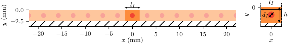
Figure 5. Infinite, periodic, phononic surface. The periodic cell (right) – clamped at the bottom and free at the top – with span l_I is periodically and infinitely replicated along the x -direction (left).
