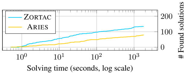
Figure 6: Coverage over 216 randomly generated instances populated with values of Table 4 (1800 seconds timeout)
