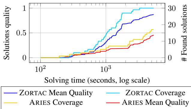
Figure 8: Solutions quality repeatability over 30 solving of a realistic instance (5400 seconds timeout)
