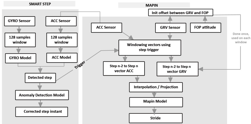
Figure 3: Algorithm of real-time implementation of MAPIN
