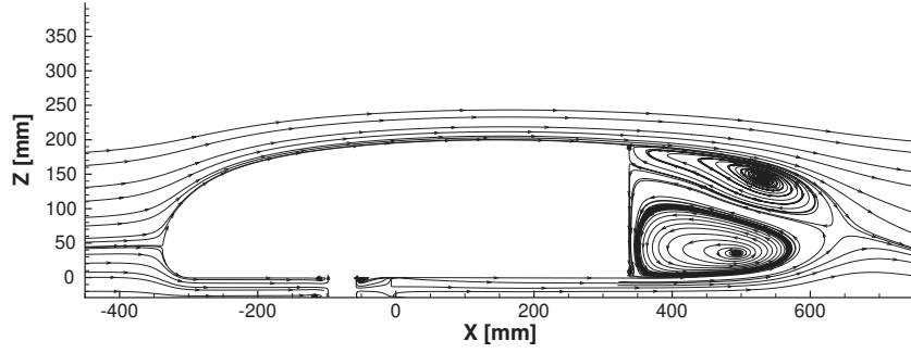
Fig. 3. \beta = 0^\circ : Streamlines in the symmetry plane.
