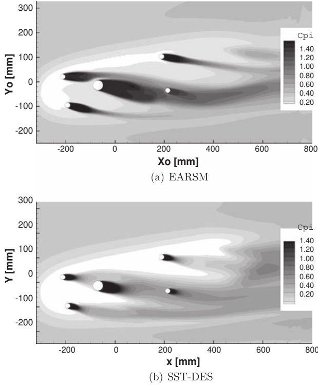
Fig. 7. Total pressure coefficient for the yaw angle \beta = 10^\circ at Z_o = -14.5 mm.
