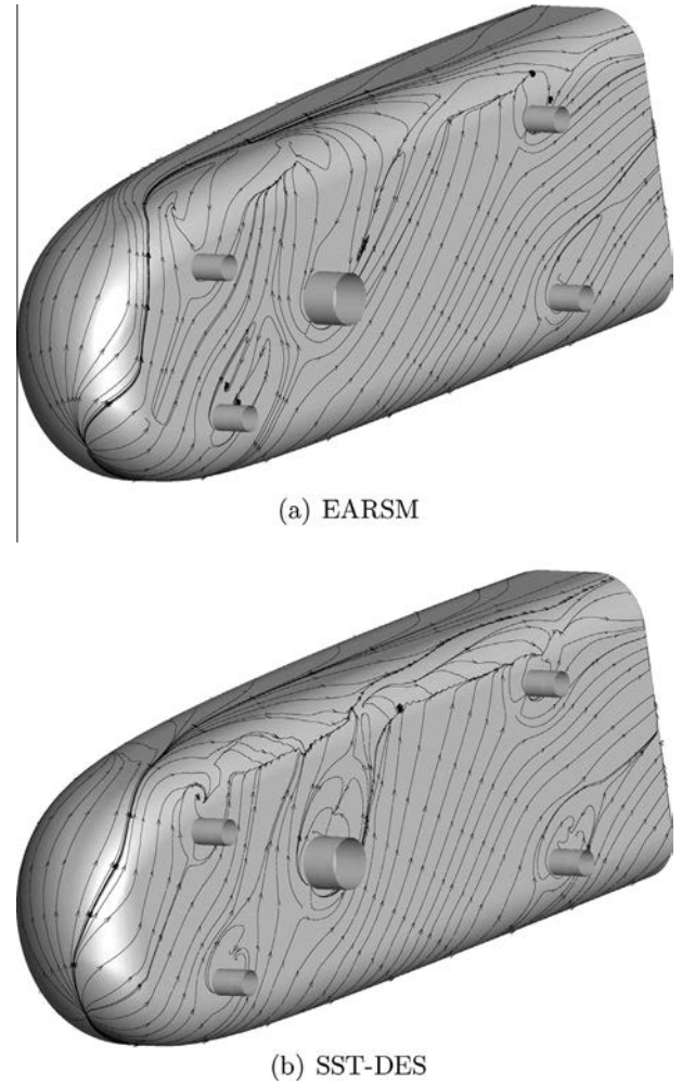
Fig. 13. Friction lines on the underbody at \beta = 30^\circ .
