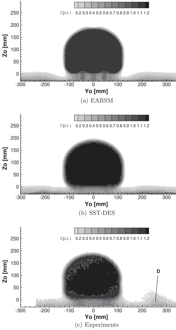
Fig. 5. Total pressure coefficient for the yaw angle \beta = 0^\circ in the Xo -plane Xo/L = 0.60 .
