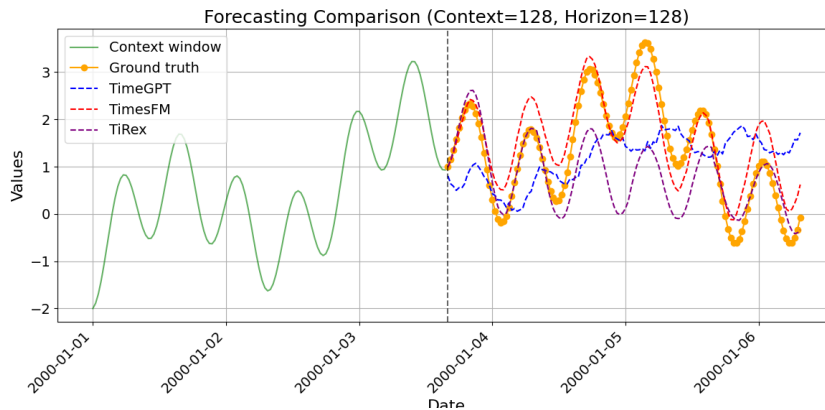
(a) Forecasting results on D1.
