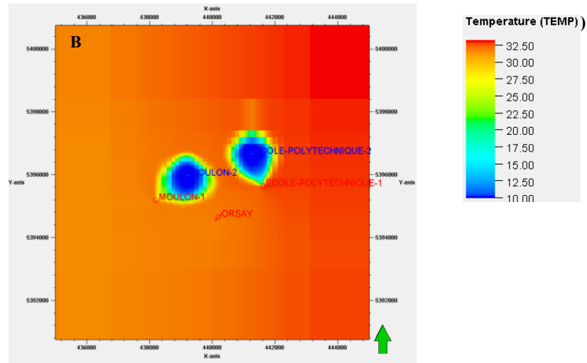
Figure 10: Cooling kinetics; A. Benchmark between ECLIPSE300, PUMAFLOW and TOUGH3 software; B. Reservoir temperature final state at year 2052
