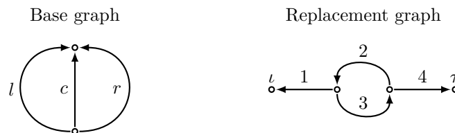
FIGURE 13. A replacement system for the Julia set of the rational map z \mapsto z^{-2} - 1 .
