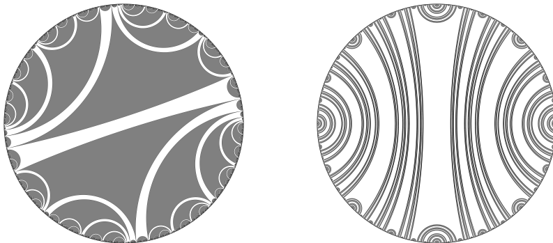
FIGURE 5. The 4-rabbit lamination and the airplane lamination.
