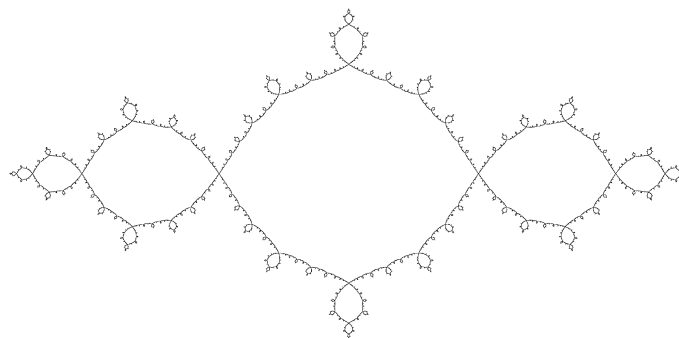
FIGURE 2. The basilica fractal.
