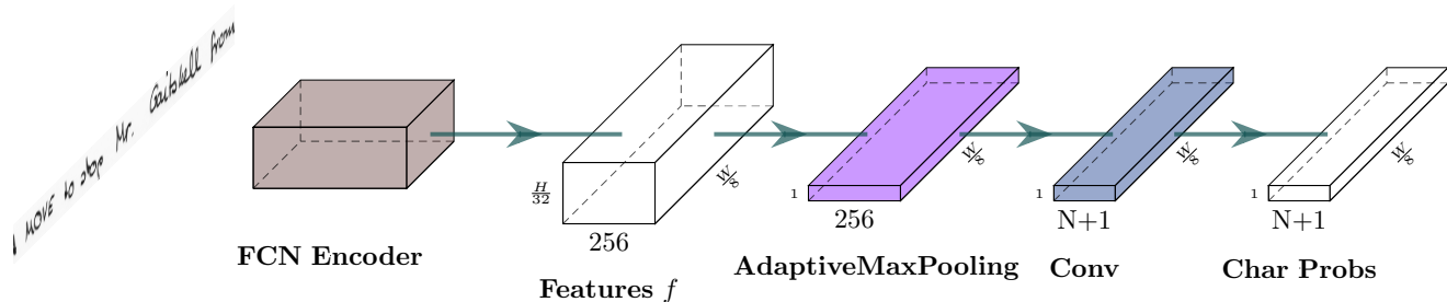
Figure 8: Text line recognition architecture overview.
