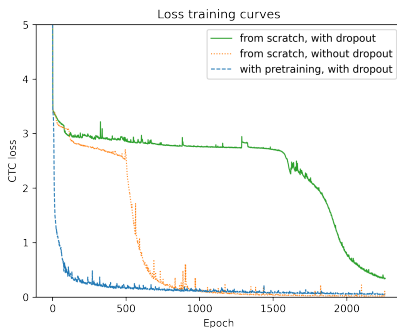
Figure 4: CTC training loss curves comparison for the VAN, with and without pretraining, on the IAM dataset.
