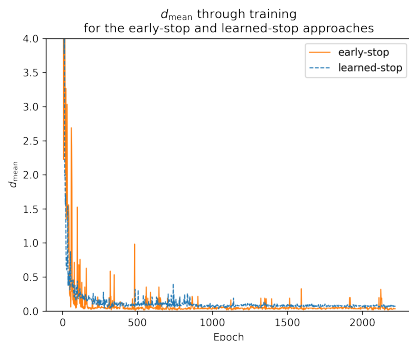
Figure 6: Comparison of the evolution of d_{\text{mean}} (the mean difference between the true and estimated number of lines in the image) on the validation set of IAM dataset for the early-stop and learned-stop approaches.
