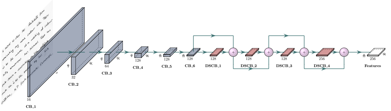
Figure 2: FCN Encoder overview. Specified dimensions are related to the output of the corresponding layer. CB: Convolution Block, DSCB: Depthwise Separable Convolution Block.
