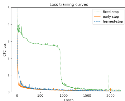
Figure 5: CTC training loss curves comparison for the VAN for each stopping approach on the IAM dataset.
