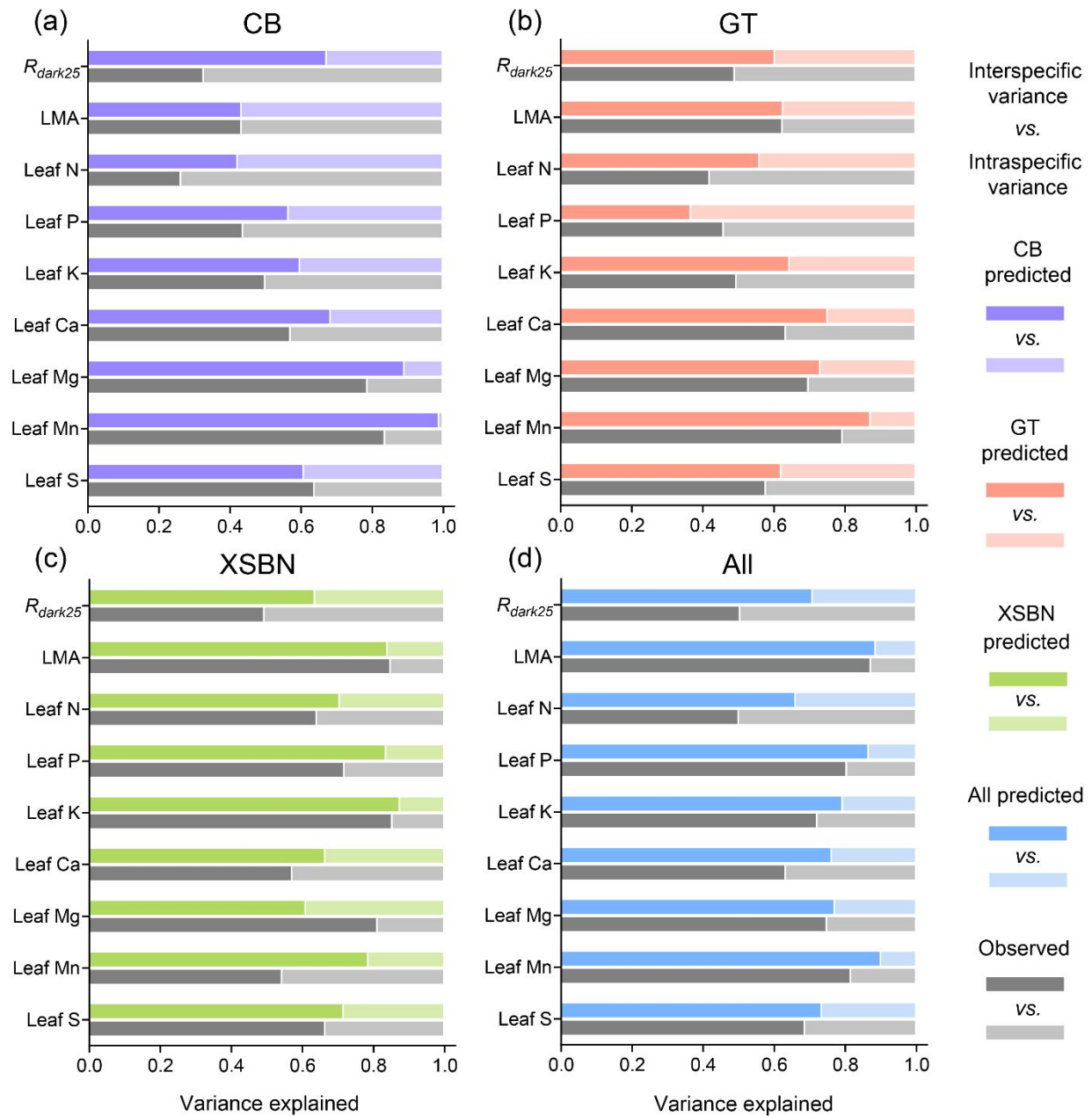
Fig. 6 Variance partitioning of leaf R_{\text{dark25}} and leaf morphological (i.e. LMA) and biochemical (i.e. leaf N, P, K, Ca, Mg, Mn and S concentrations) traits within (a-c) and across forest sites (d). The forest sites include the temperate forest in CB, the subtropical forest in GT, and the tropical forest in XSBN in China. The total variability for each trait was partitioned into intraspecific and interspecific components. The grey bars denote the variance partitioning from field-observed leaf traits, while the colored bars indicate the variance partitioning results from leaf traits predicted from the cross-site spectra-trait models.
