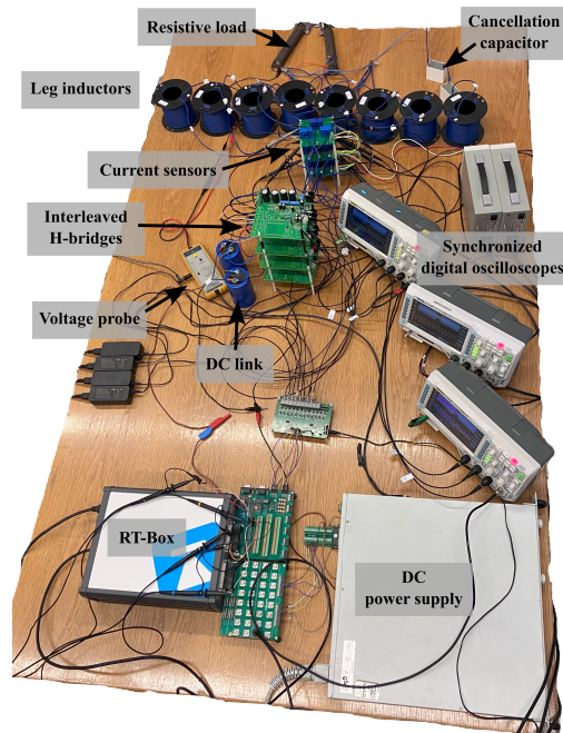
Fig. 8. View of the whole experimental setup.
