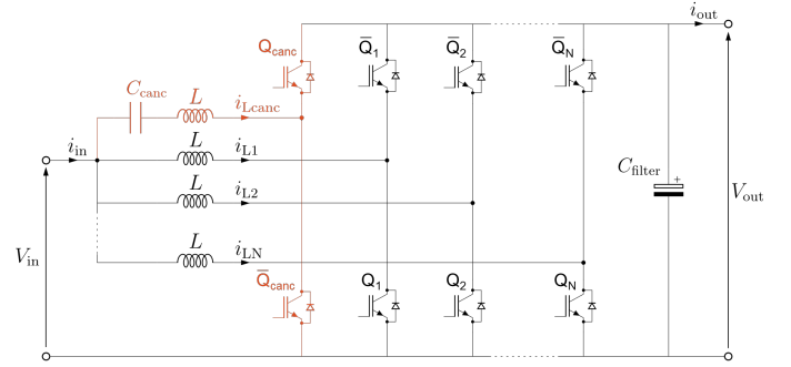
Fig. 1. Generic circuit diagram of a stacked interleaved synchronous boost converter with N legs. The cancellation leg is highlighted in red.
