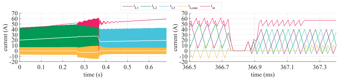
Fig. 7. Power legs, cancellation, and input currents under active leg number rearrangement from N' = 2 to N'' = 3 . The right frame shows a detailed view of the currents during the leg transition. White lines on the left frame are the moving average of power legs and cancellation currents.
