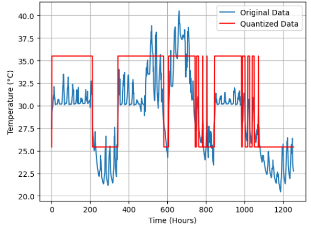
Fig. 2. Temperature time series from the Twin House Experiment (sensor in the living room at a height of 10cm) and corresponding quantization based on \rho_{0.1} , corresponding to \alpha = 0.1 in (18).
