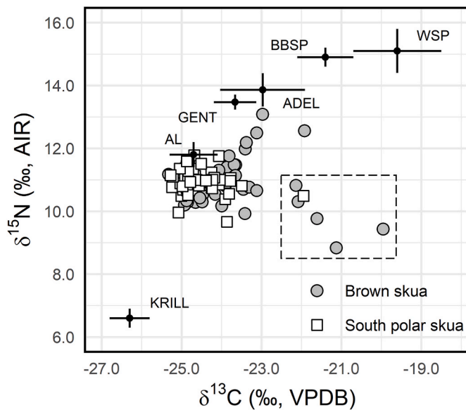
Fig. 3. Individual stable isotope values (‰) of carbon ( \delta^{13}\text{C} ) and nitrogen ( \delta^{15}\text{N} ) in red blood cells of breeding brown skuas Stercorarius antarcticus lombergi (circles) and south polar skuas S. macormicki (squares) from the Potter Peninsula, King George Island (Isla 25 de Mayo), South Shetland Islands, Antarctica. Mean ( \pm SD) \delta^{13}\text{C} and \delta^{15}\text{N} values of potential prey (lipid extracted) are also shown, including Antarctic krill Euphausia superba (KRILL), Antarctic lanternfish Electrona antarctica (AL), eggs of Adélie penguins Pygoscelis adeliae (ADEL) and gentoo penguins P. papua (GENT) and Wilson's storm petrel Oceanites oceanicus (WISP) and black-bellied storm petrels Fregetta tropica (BBSP) (Cipro et al., 2017; Polito et al., 2016; Graña Grilli et al., 2023; Quillfeldt et al., 2023). Trophic enrichment factors are applied to prey values following Graña Grilli et al. (2023). Dashed rectangle indicates individuals using an alternative trophic pathway (see text).
