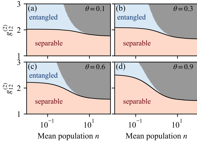
FIG. 4. Entanglement regions in the (n, g_{12}^{(2)}) plane, for a given value of \theta in each panel. Compared to the entanglement witness shown in Fig. 3, there is no unknown entanglement region.
