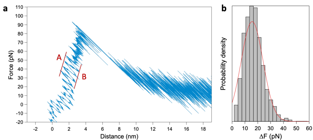
Figure 5. a. Characteristic force–distance profile obtained for M1 at a pulling rate of 20 \text{ nm}\cdot\text{s}^{-1} . b. Histogram of the amplitude of the fluctuations ( \Delta F ) (red trace: Gaussian Fit). N=1681 .
