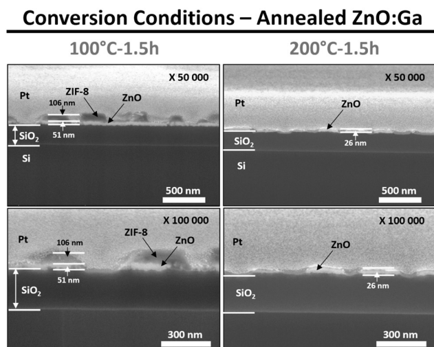
Fig. 8 SEM observations (cross-sections) of annealed ZnO:Ga samples after reaction/conversion in a CH 3 OH/H 2 O mixture (3:1) at different reaction temperatures (100 °C and 200 °C) for 1.5h.
