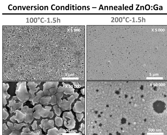
Fig. 7 SEM observations (surfaces) of annealed ZnO:Ga samples after reaction/conversion in a CH 3 OH/H 2 O mixture (3:1) at different temperatures (100 °C and 200 °C) for 1.5 h.
