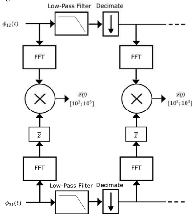
Fig. 4. Architecture of the FPGA signal processing.
