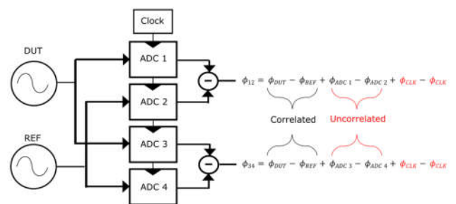
Fig. 3. Cross-spectrum experimental method.
