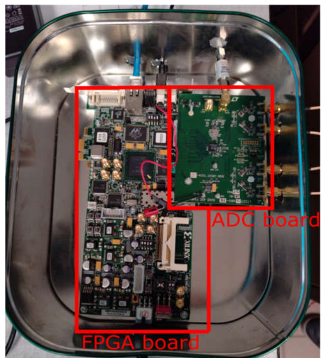
Fig. 2. AH analyzer.
