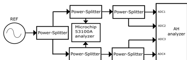
Fig. 6. Schematic of the noise floor measurement setup.
