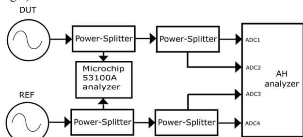
Fig. 5. Simplified schematic of the PSD measure setup.
